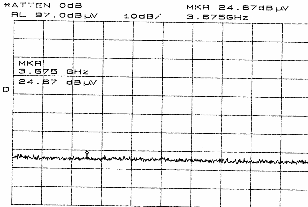
Figure sixteen Radiated Emissions in screen room (BT Tx).
