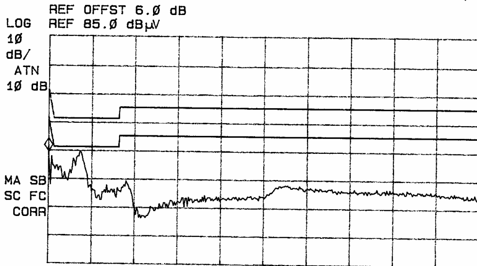
Figure three Conducted emissions of EUT line 1 (ADP-5FH B)
