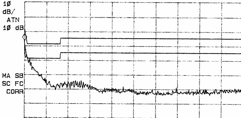
Figure seven Conducted emissions of EUT line 1 (CPU)
