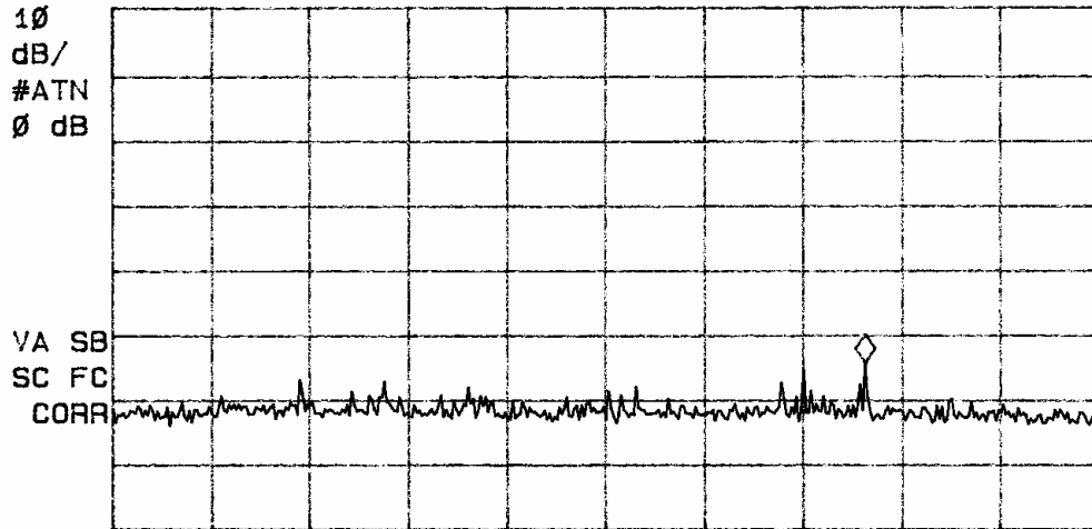
Figure thirteen Radiated Emissions in screen room (BT Tx).
