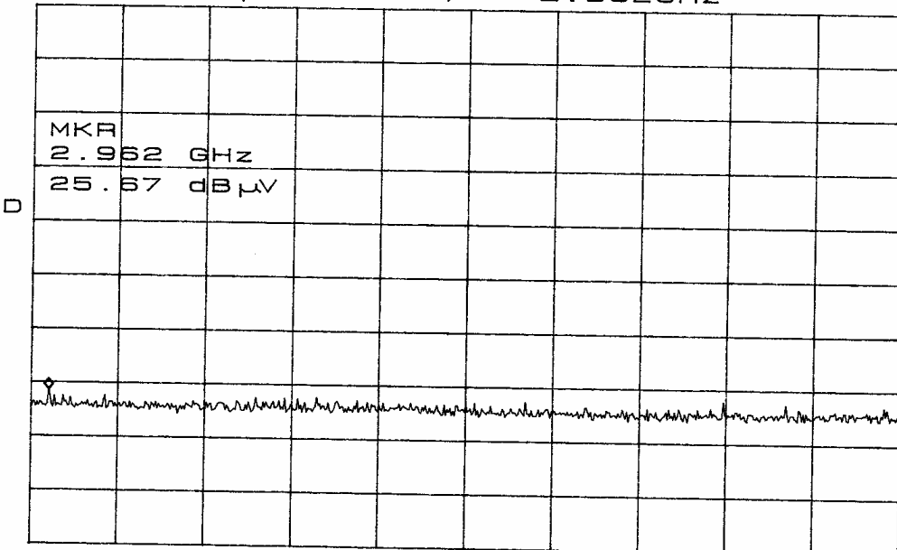
Figure twelve Radiated Emissions in screen room (FM Tx).
