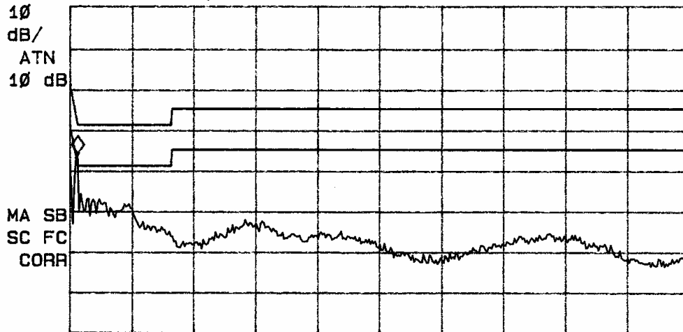
Figure Six Conducted emissions of EUT line 2 (PSC05R-050A1)
