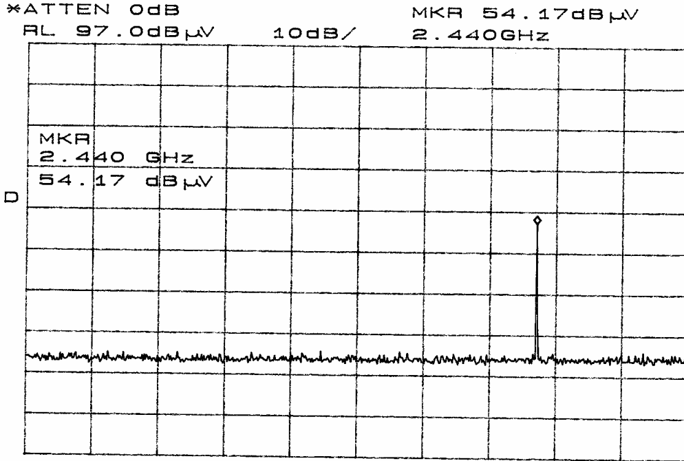
Figure fifteen Radiated Emissions in screen room (BT Tx).
