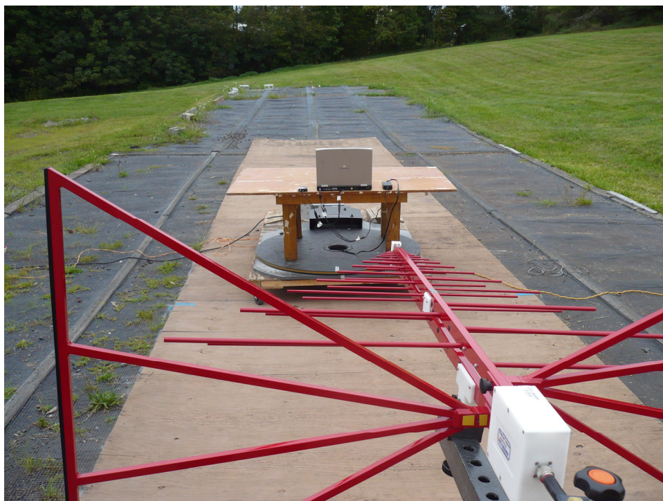
Horizontal Biconical Antenna Polarization
