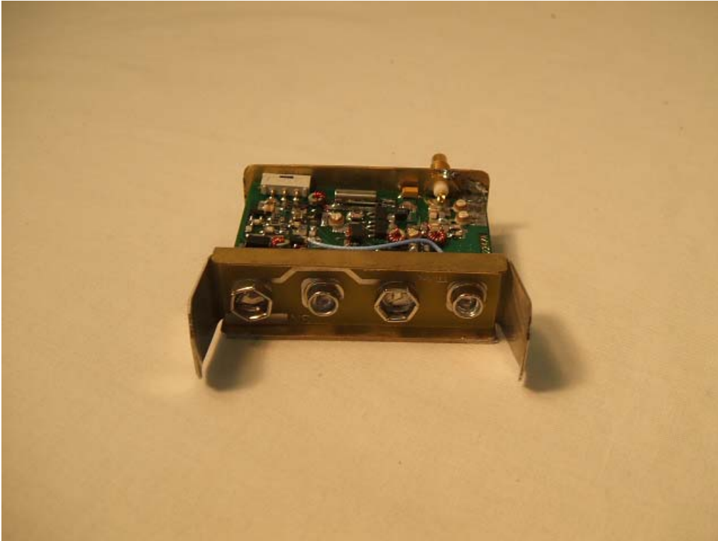
IP9J1W both boards mounted in enclosure
