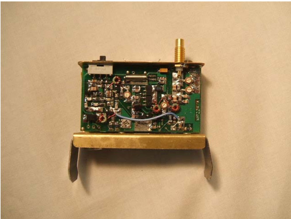
IP9J1W RF Board mounted in enclosure
