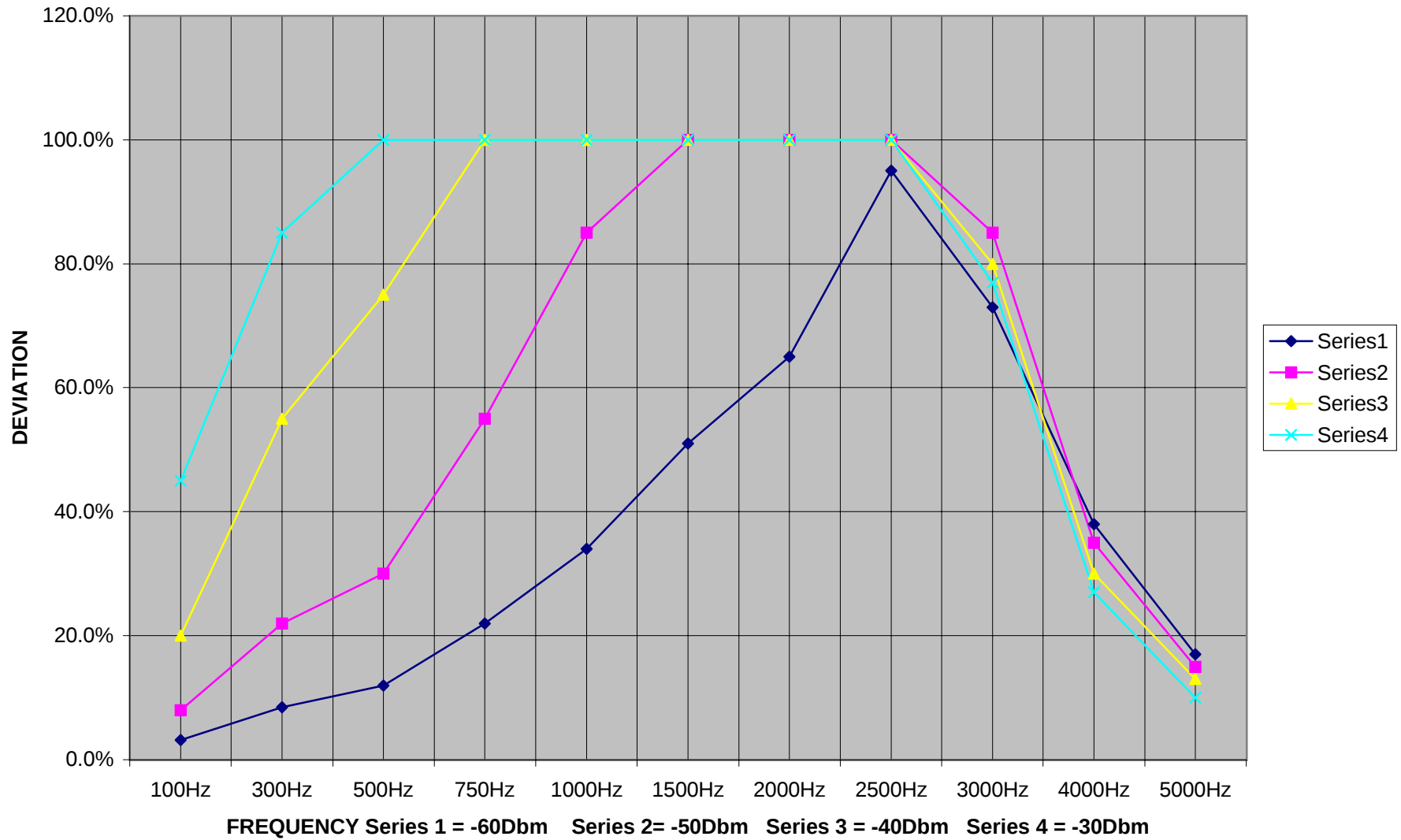
INPUT SIGNAL LEVEL VS. DEVIATION ECHO TX FCC ID # IP9ECHO-TX9A
