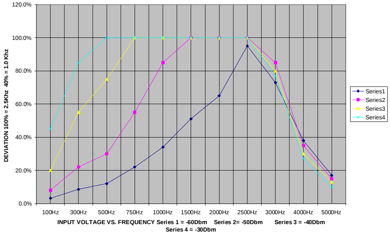
INPUT SIGNAL LEVEL VS. DEVIATION CST-751/V FCC ID # IP9751V
