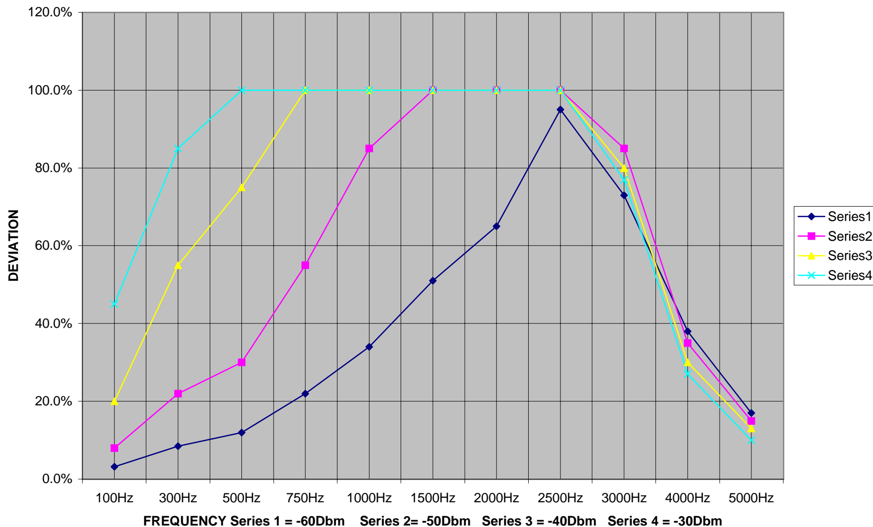
INPUT SIGNAL LEVEL VS. DEVIATION CST-2001/V FCC ID # IP92K1V
