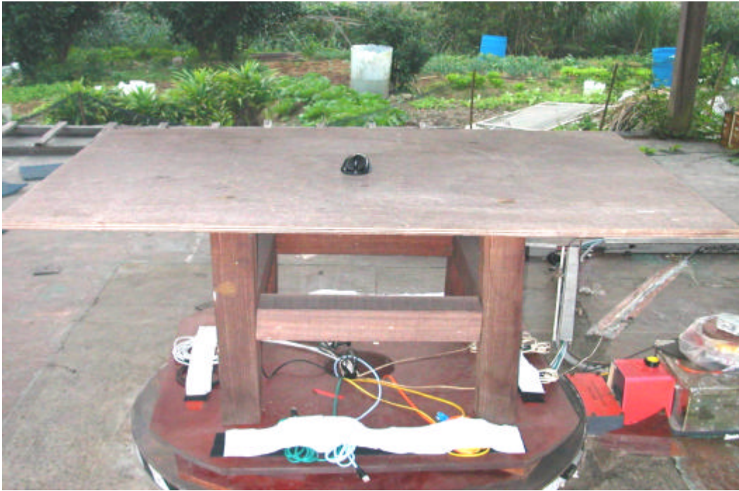
Front View of the Test Configuration
