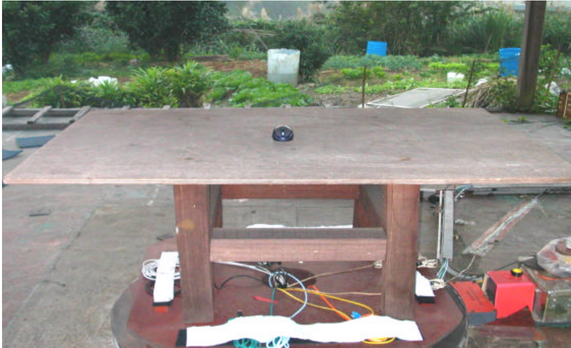
Front View of the Test Configuration
