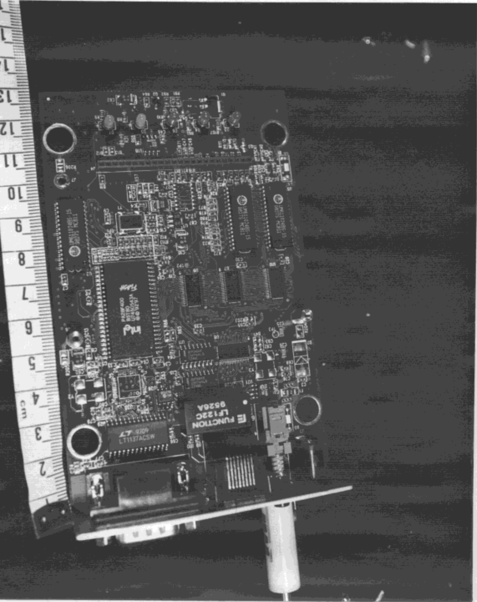
Top side view of Main board-2
