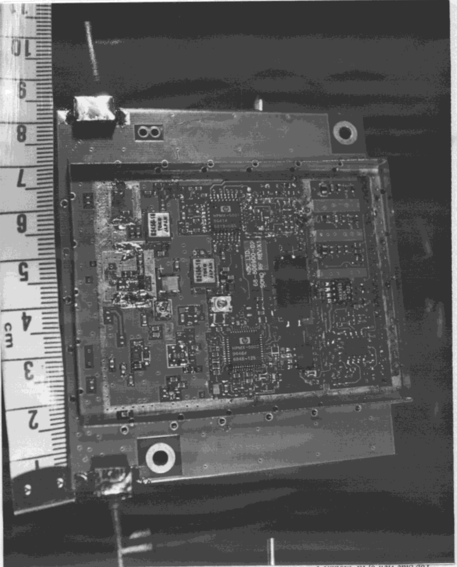
Top Side view of RF Module-3
