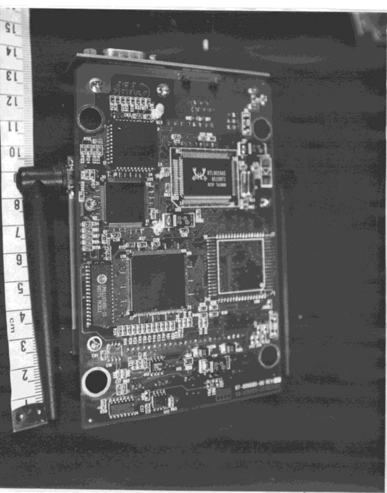
Back side View of Main board
