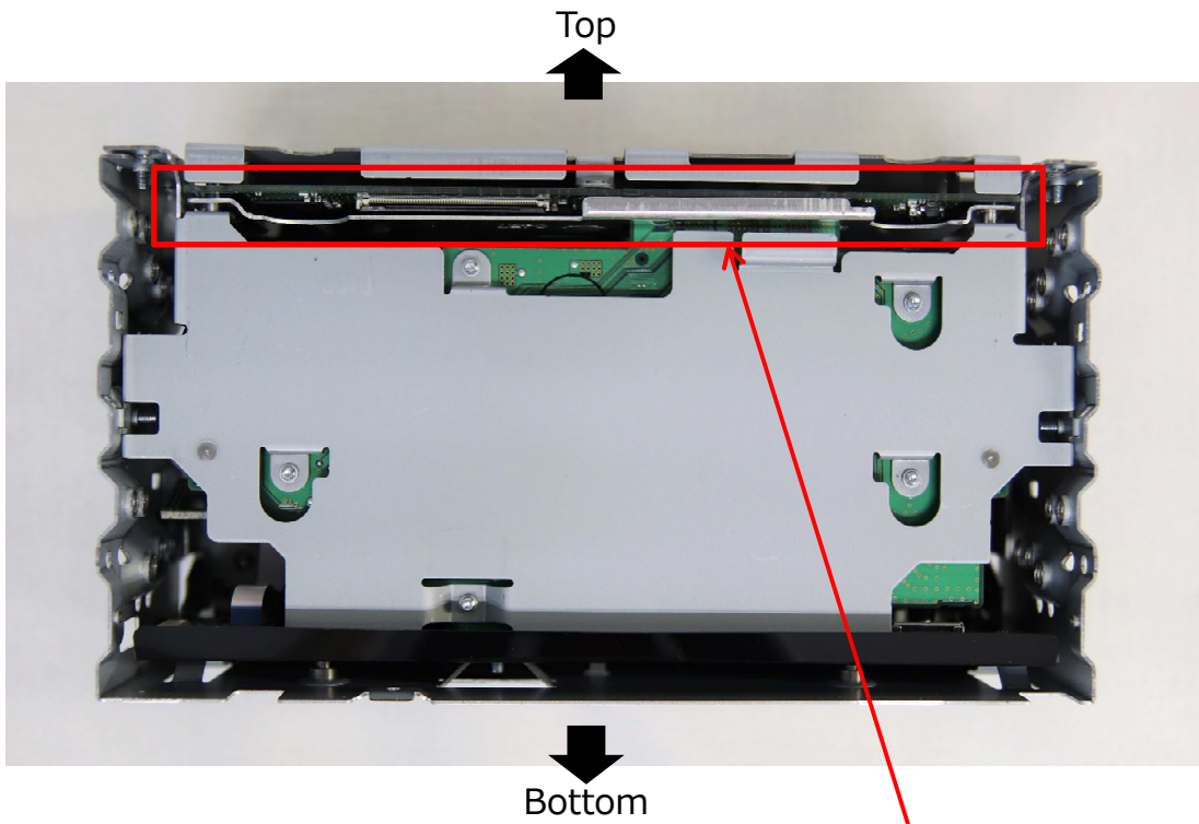
PCB with Radio module covered by shield plate
