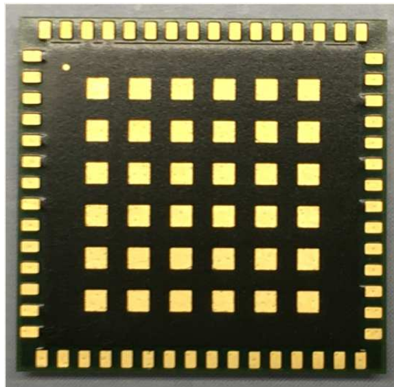
Radio Module (B-side)
