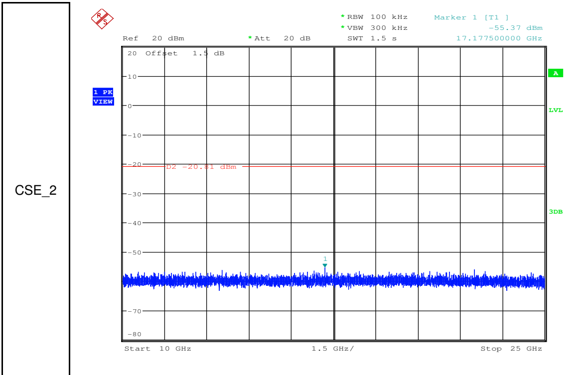
RF Conducted Spurious Emissions_11N40SISO_2422_Ant1
