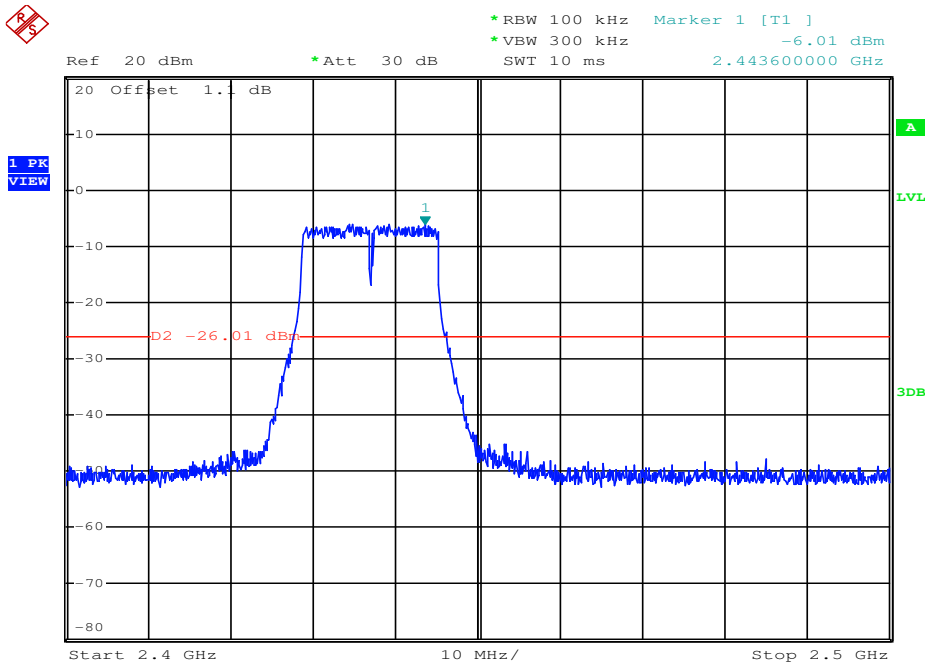
RF Conducted Spurious Emissions_11N20SISO_2437_Ant1
