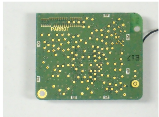
BT Transmitter 2
