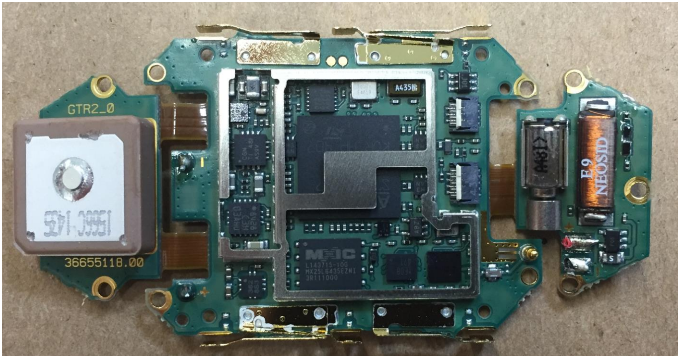
Figure 7. PWB module shield removed, top view.
