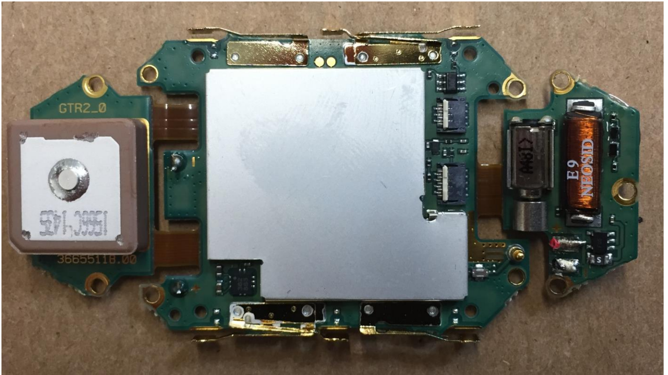
Figure 5. PWB module, top view
