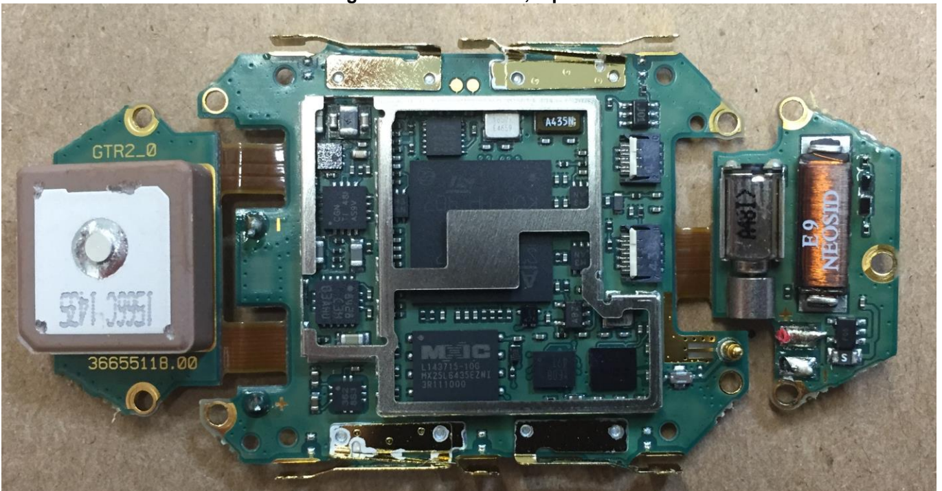
Figure 6. PWB module shield opened, top view.
