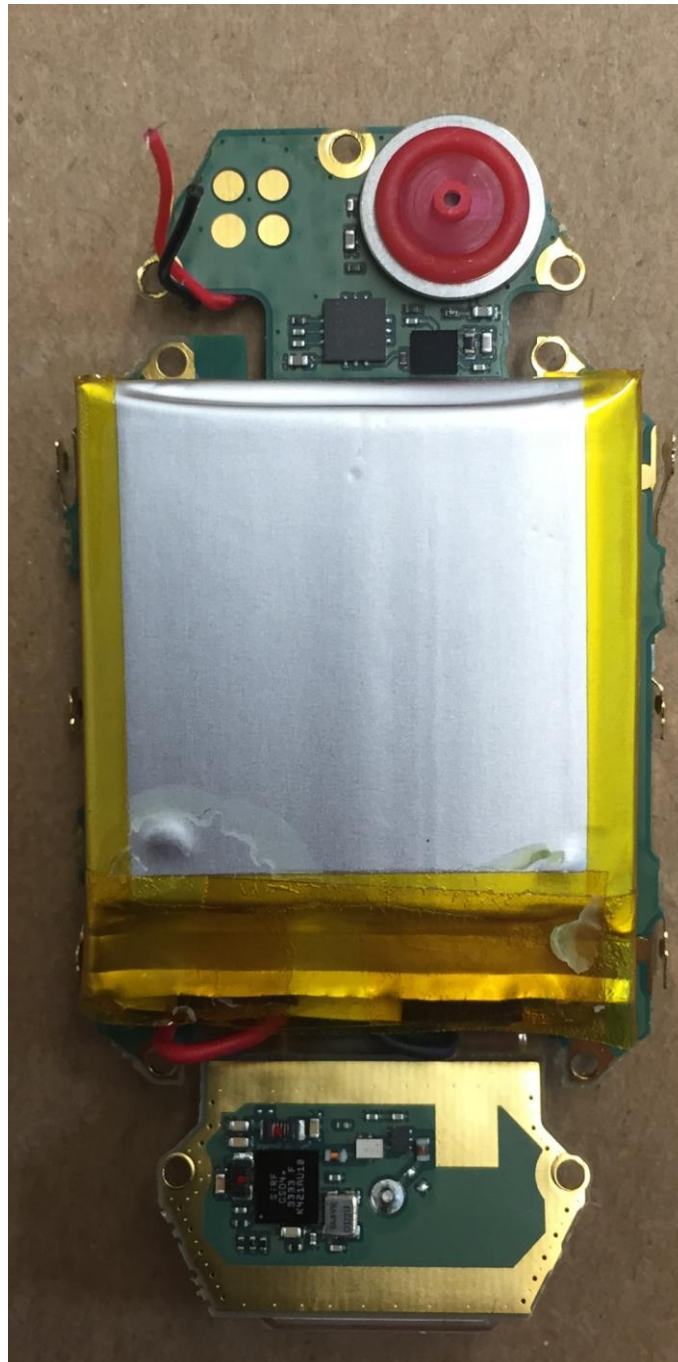
Figure 4. Electronics module from the back side. Battery on top of PWB.
