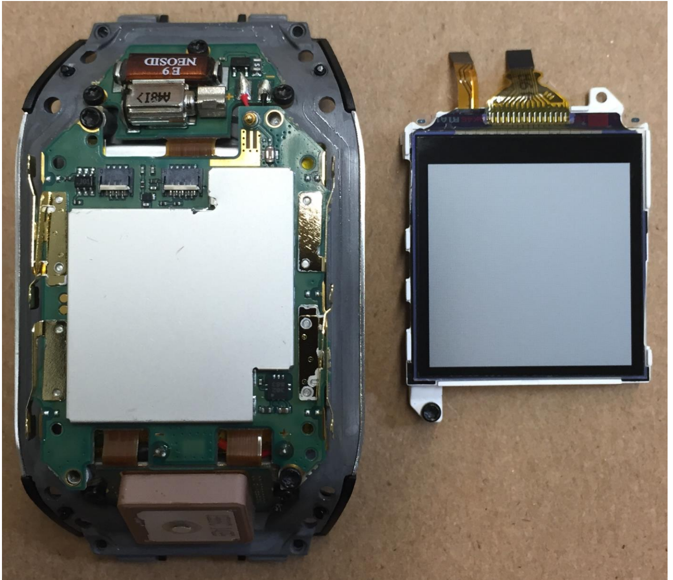
Figure 2. Display detached.
