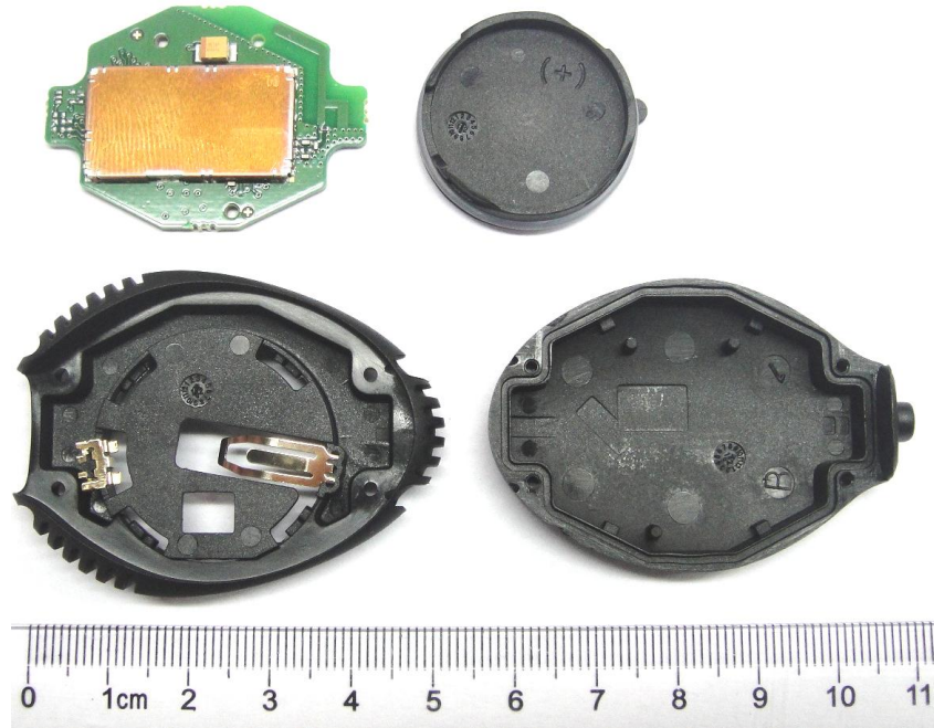
Figure 1. Product opened
