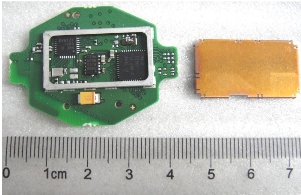
Figure 2. PWB top side, shield opened
