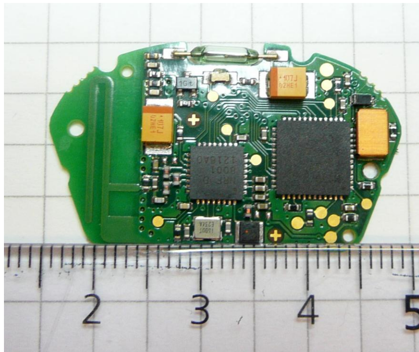
Figure 3. PWB top side
