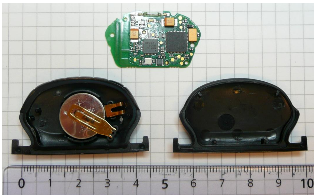
Figure 2. PWB removed from the cover
