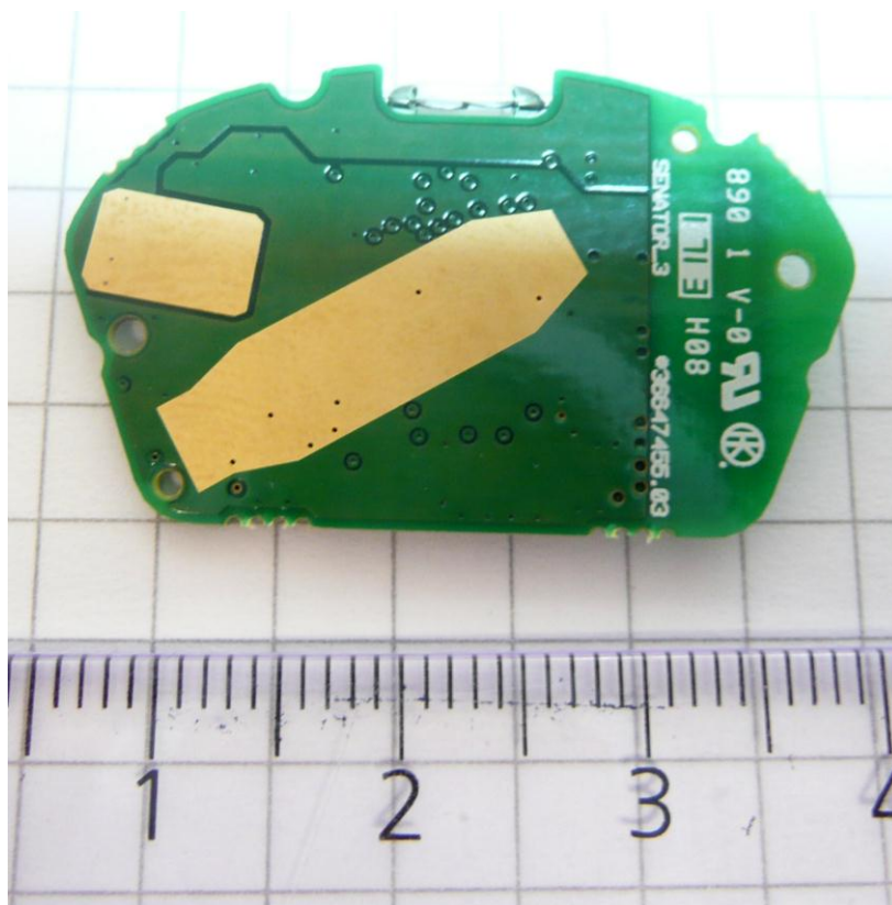
Figure 5. PWB bottom side
