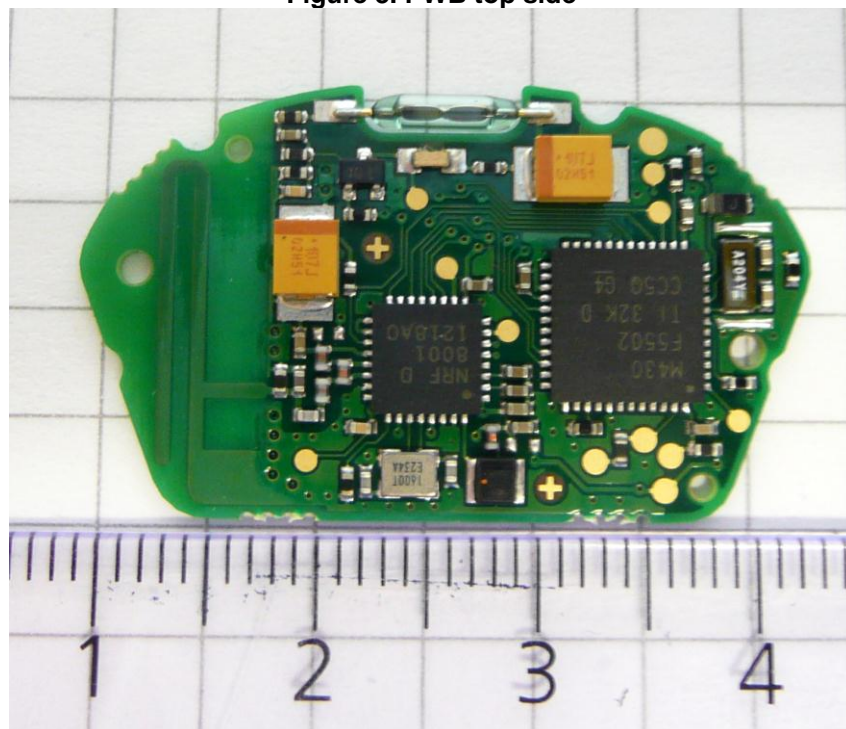
Figure 4. PWB top side, shield removed.
