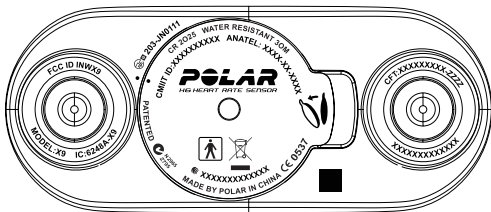
Reference backside Maximum situation for markings
