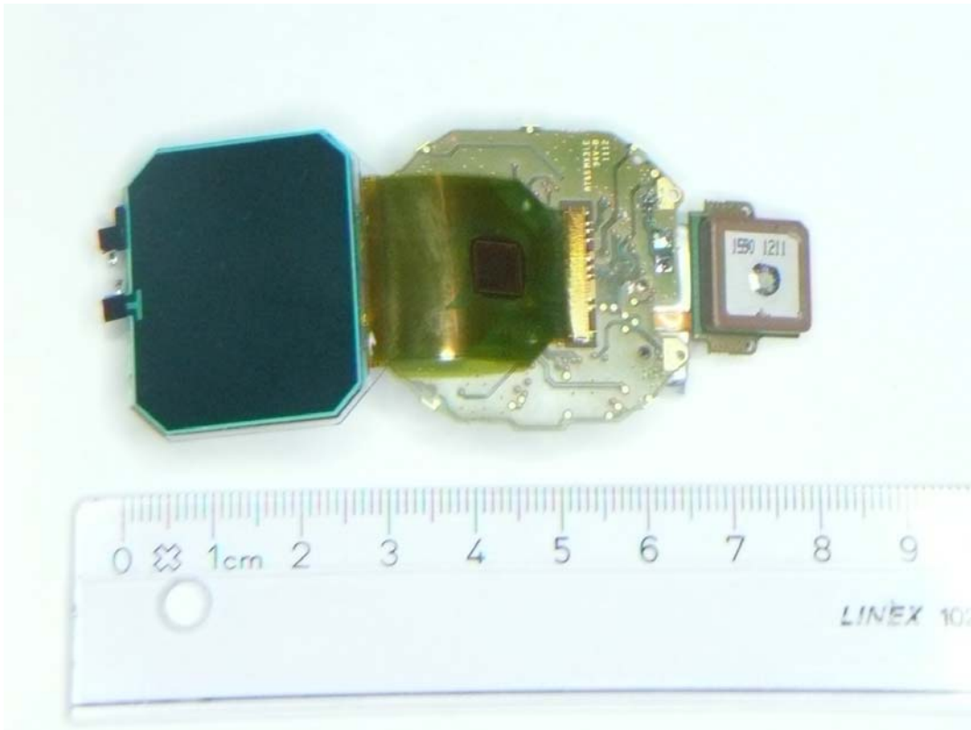
PWBA Front view
