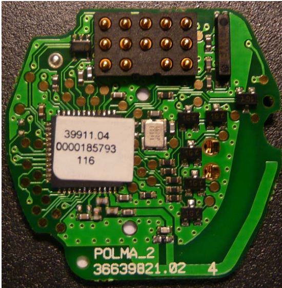
Master main board top
