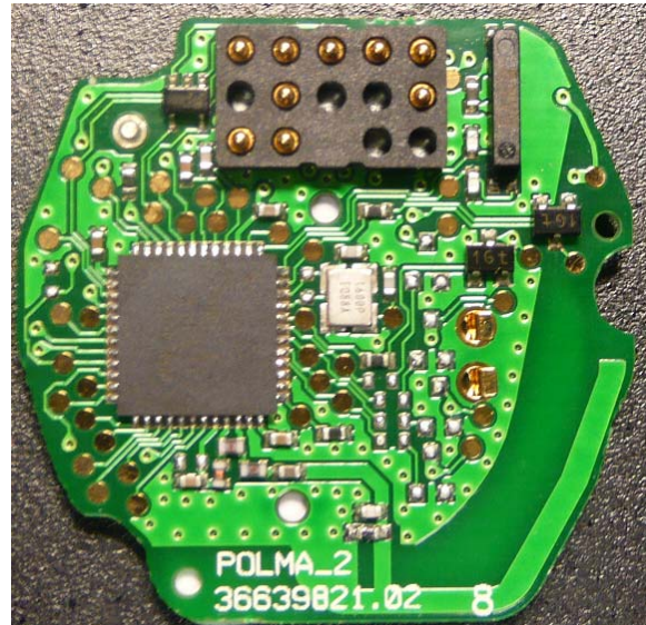
Slave main board top
