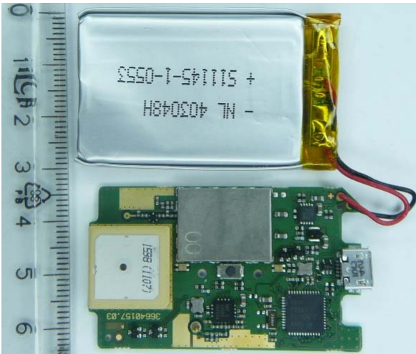
Sensor disassembled, rear view.
