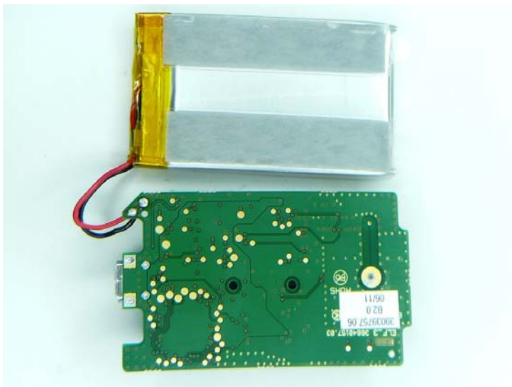
Sensor disassembled, rear view.
