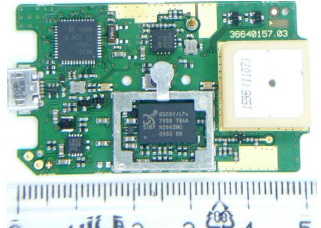
And front view with RF shield opened.
