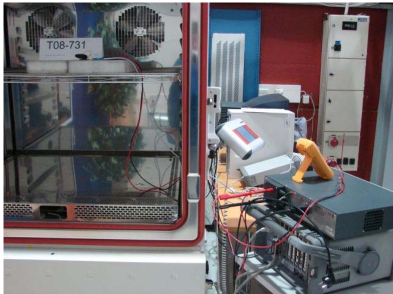
Picture 1: Conducted and extreme conditions test setup
