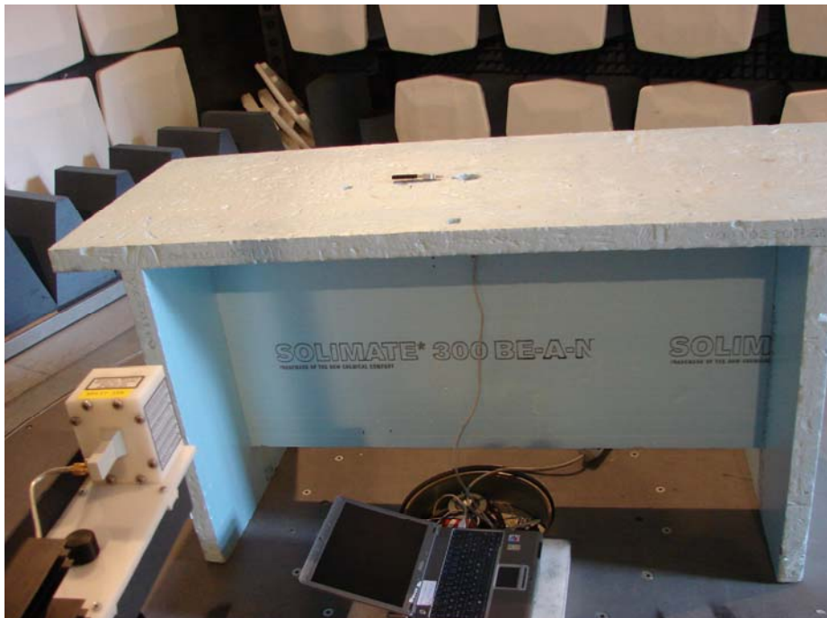
Picture 2: Spurious emission measurement setup
