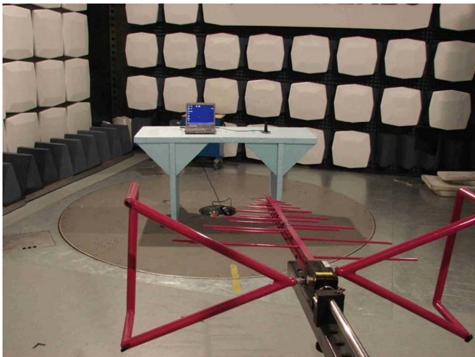
Picture 2: Radiated spurious test setup 30 MHz-140 MHz
