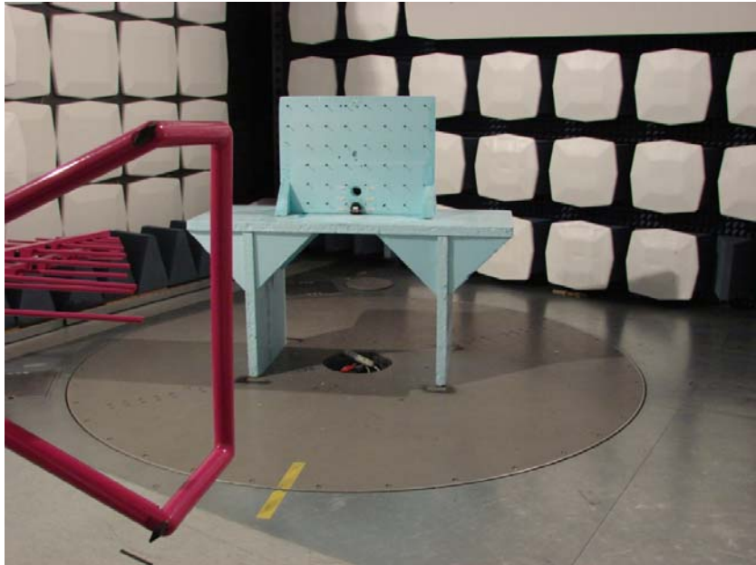
Picture 1: Spurious emission measurement setup
