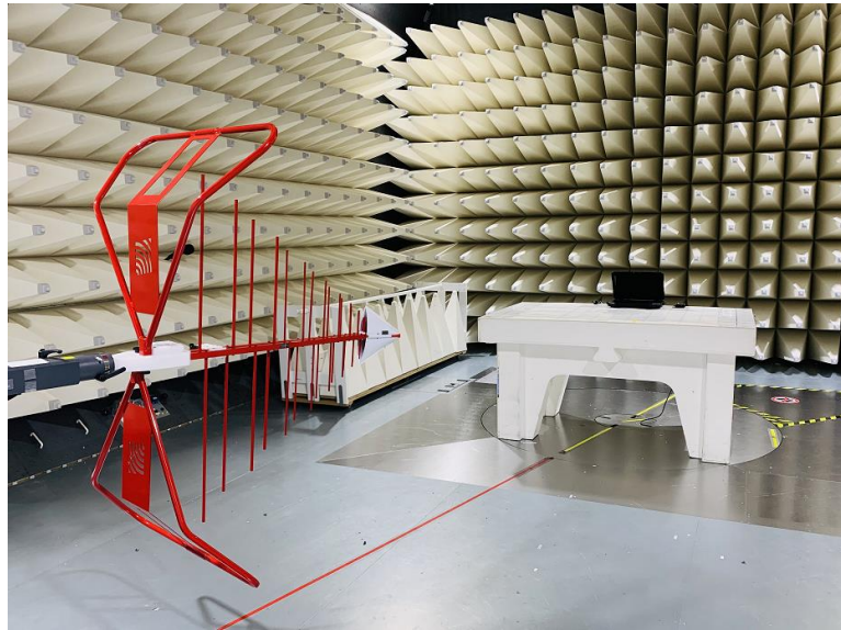
Figure B3. Low Range Radiated Emission Setup
