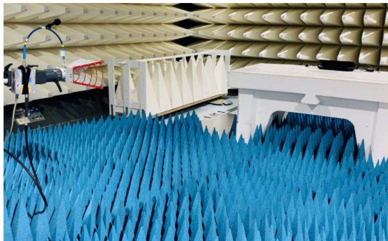
Figure B4. High range Radiated Emission Setup
