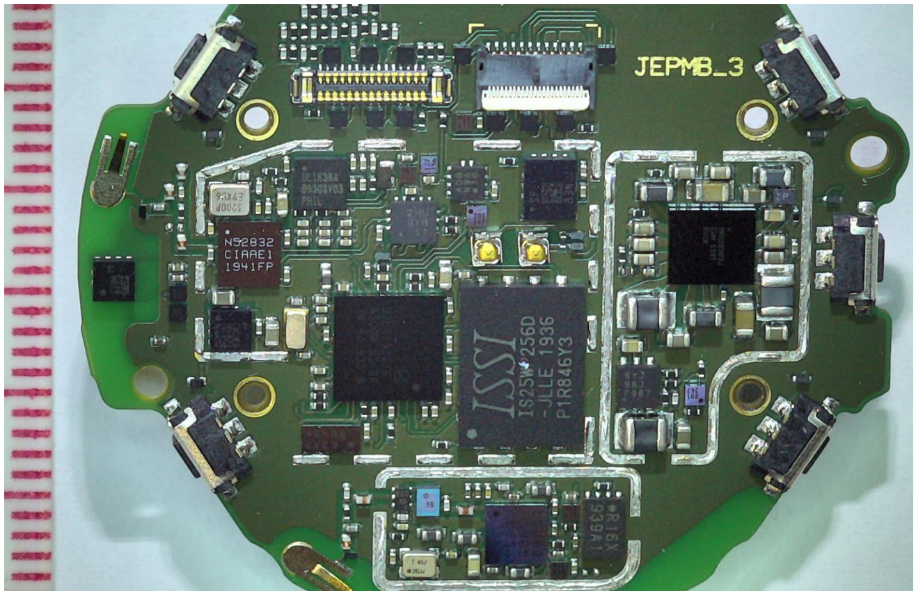
Figure 7. PWB from component side without RF shields.
