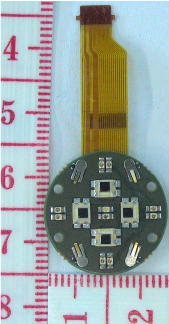
Figure 11. OHR PWB from LED side.
