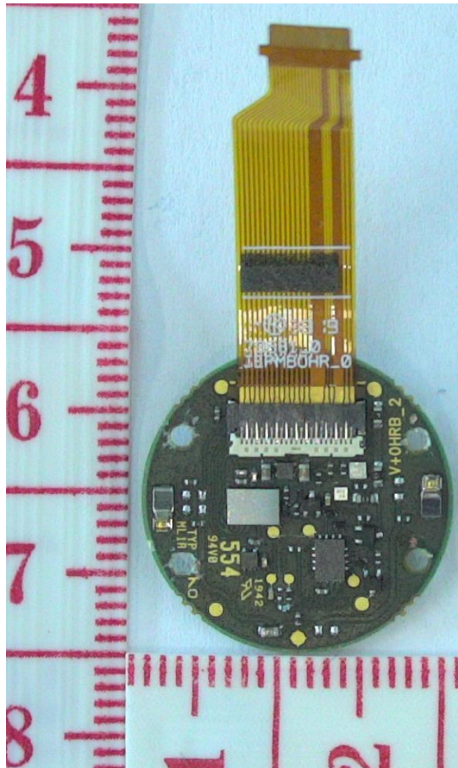
Figure 12. OHR PWB from component side.
