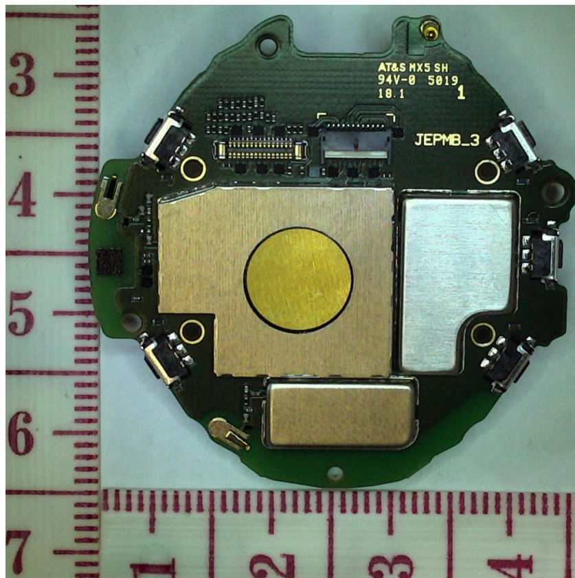
Figure 5. PWB from component side.
