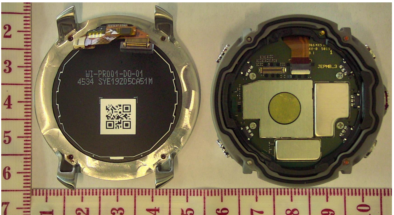
Figure 2. Display module and HW part with back case separated.
