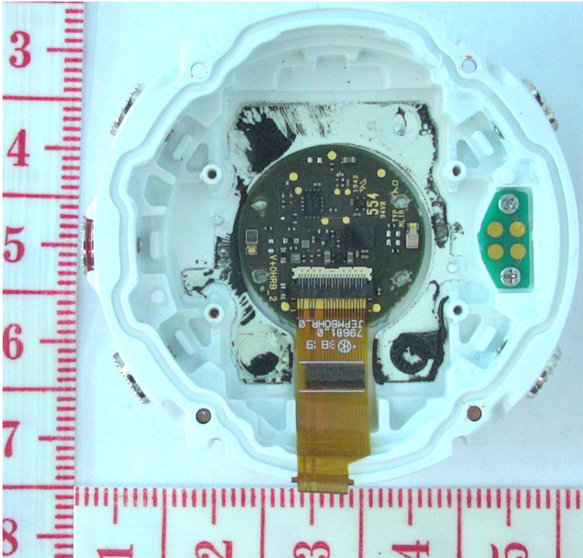
Figure 10. Optical heart rate PWB in its place.
