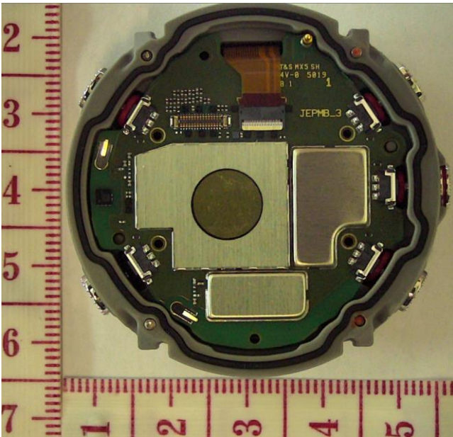
Figure 3. PWB in back case.
