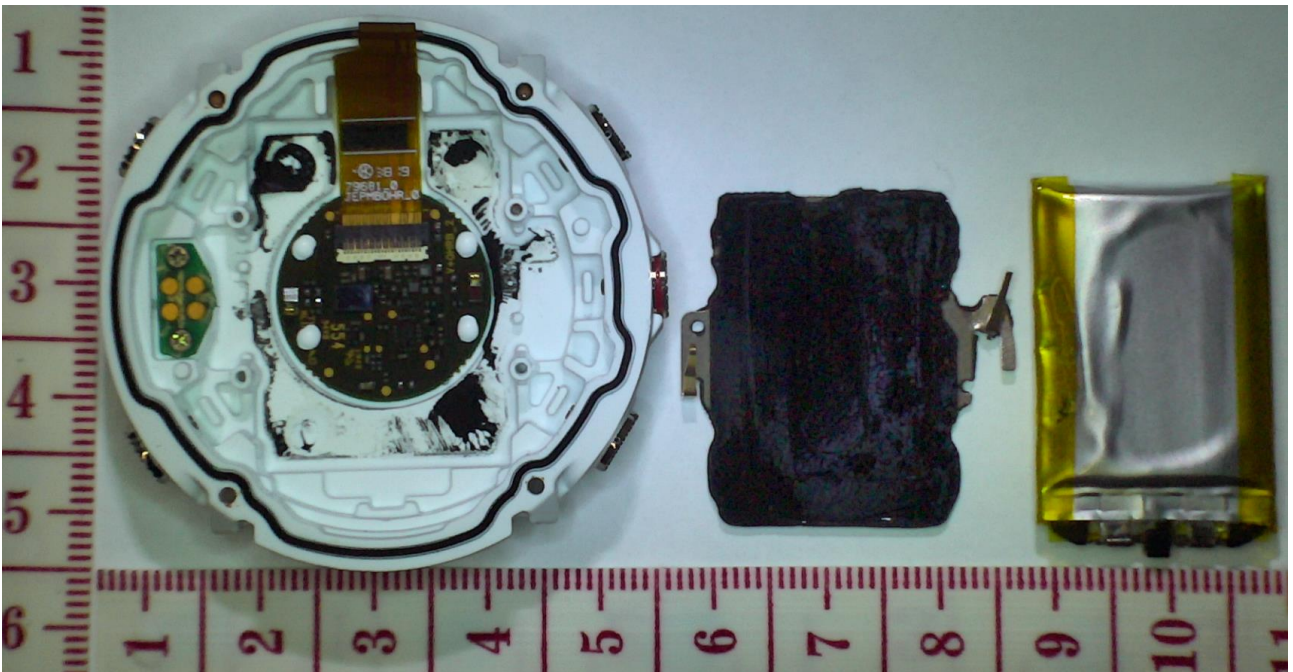
Figure 9. Battery removed from back case. Plate battery assembly in the middle.
