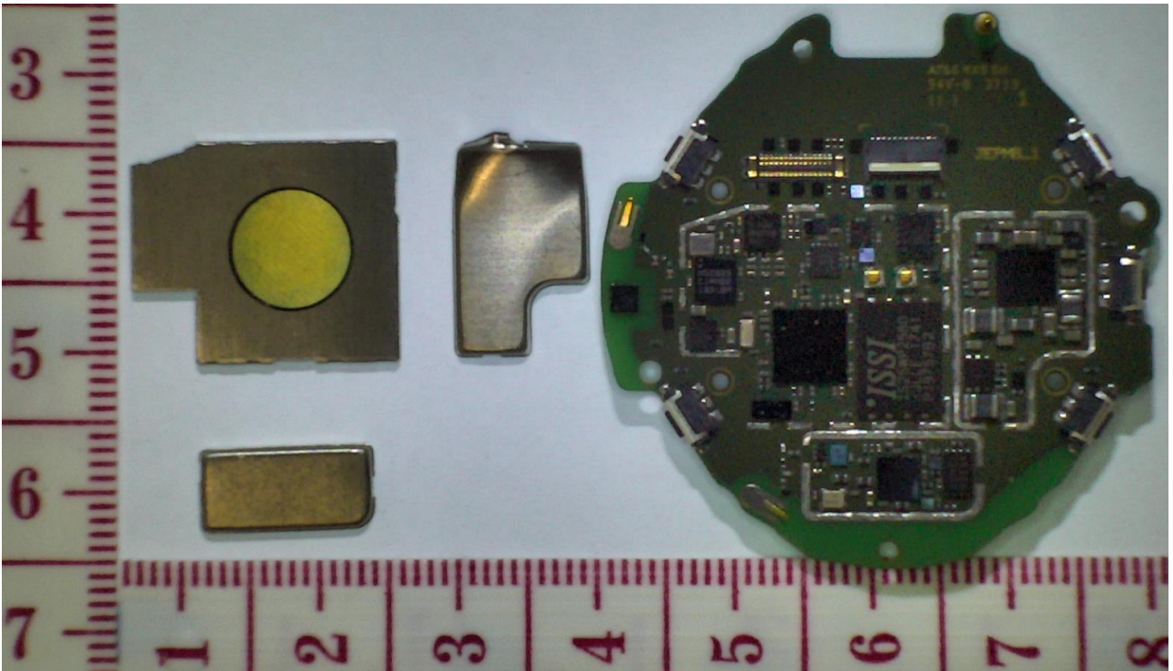
Figure 8. PWB with separated RF shields
