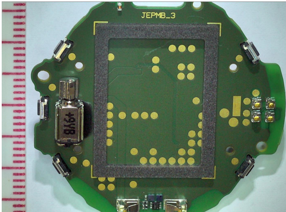
Figure 6. PWB from other side. Vibra motor on left hand side.
