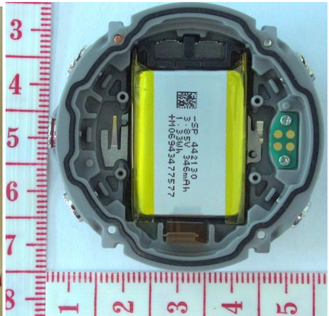
Figure 4. PWB removed, battery in back case.
