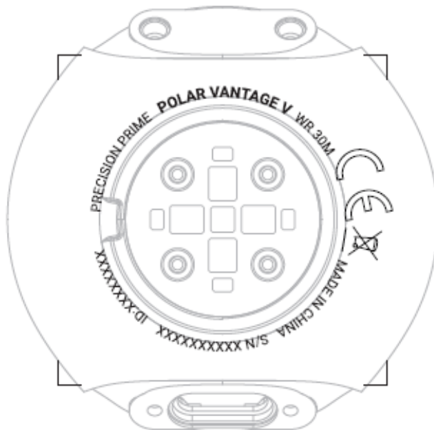
Laser markings position
