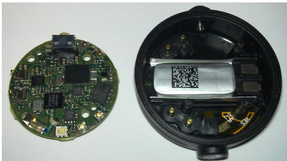
Figure 3. The PWB removed, the other side of the PWB.
