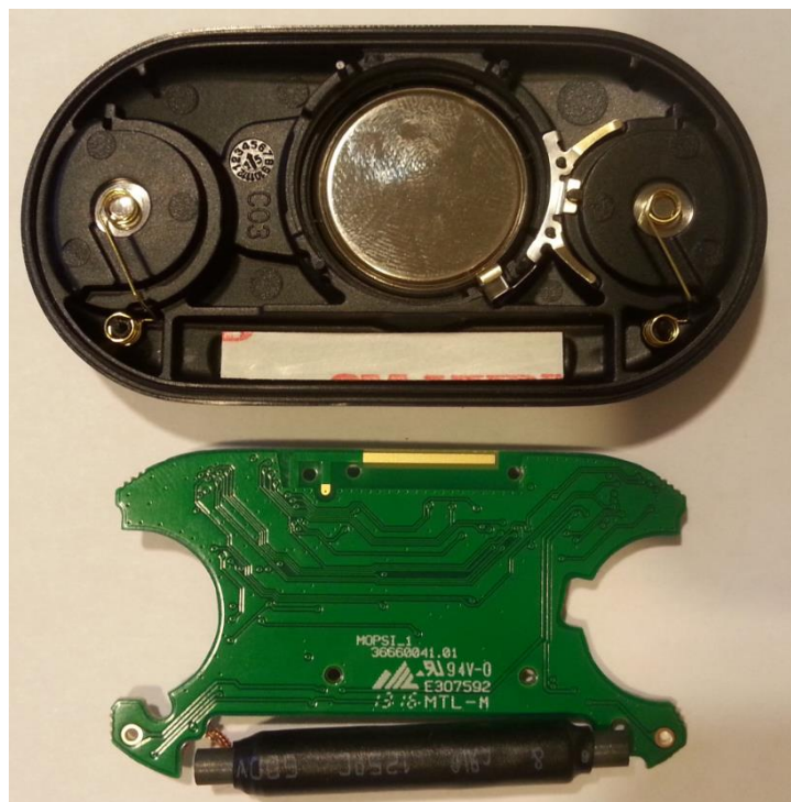
Figure 2. PWB removed from the back cover.
