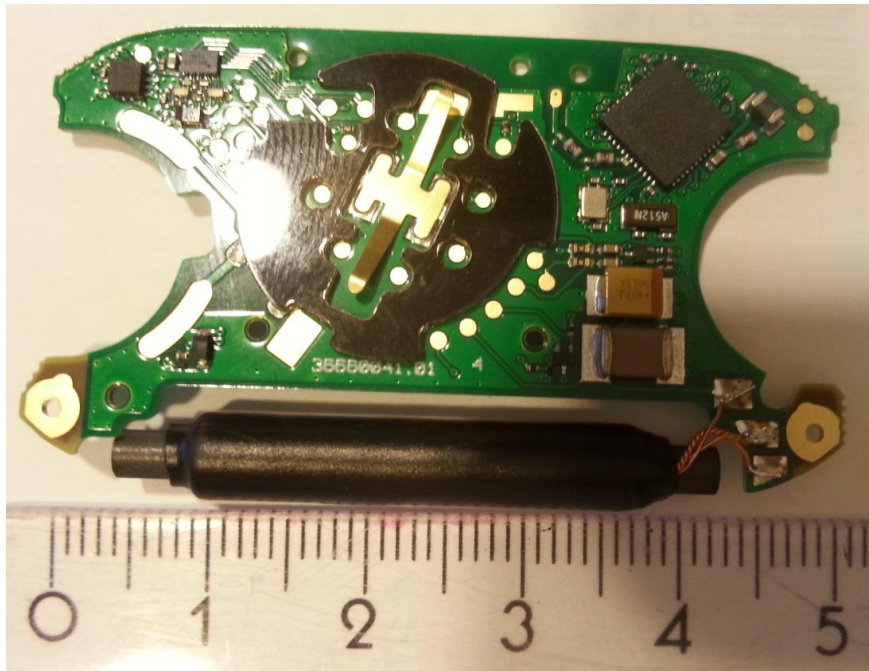
Figure 3. PWB module, top side.
