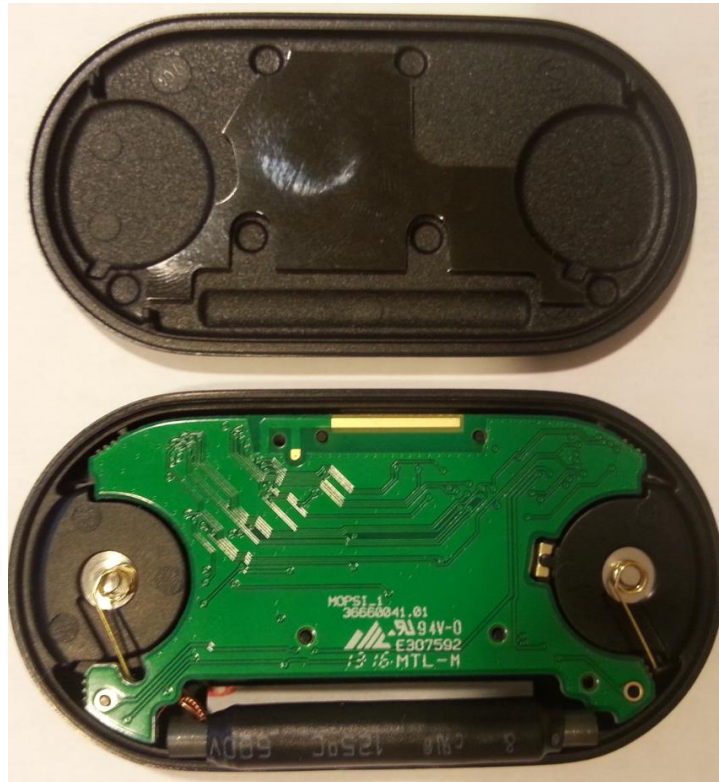
Figure 1. Front cover opened
