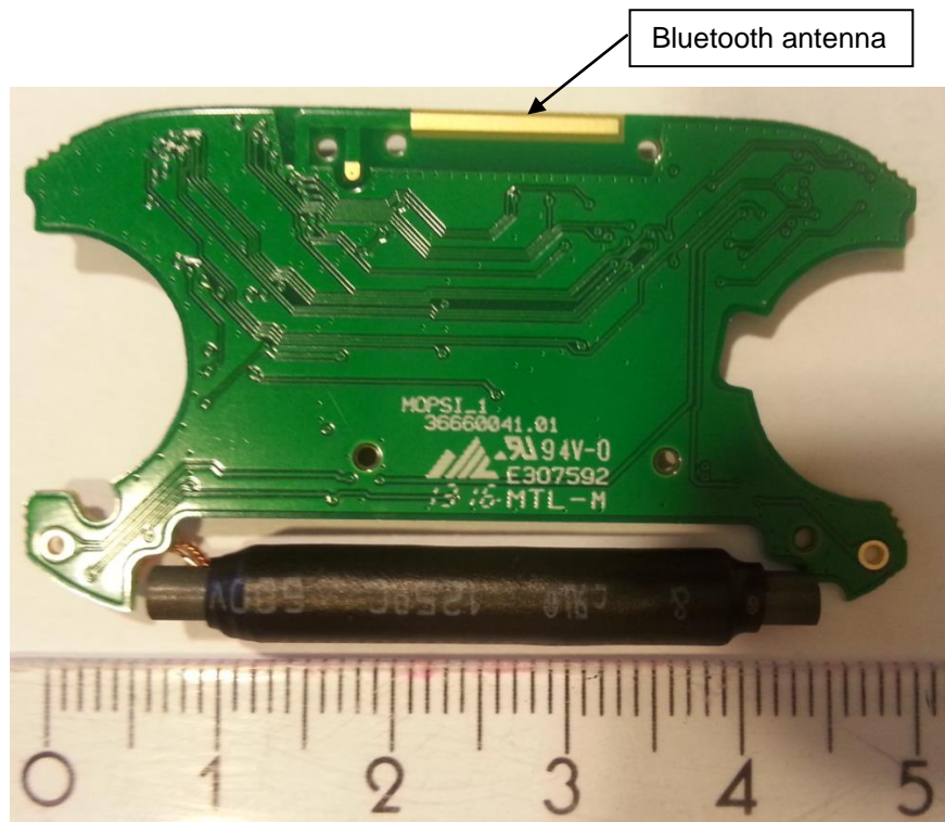
Figure 4. PWB module, bottom side.
