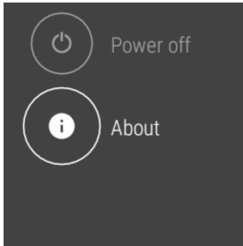
Figure 3. Select "About"
