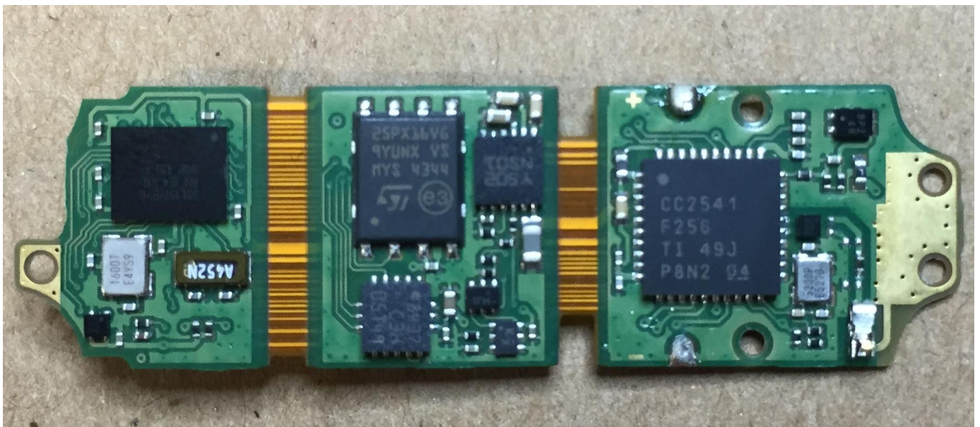
Figure 6. PWB module, top side.
