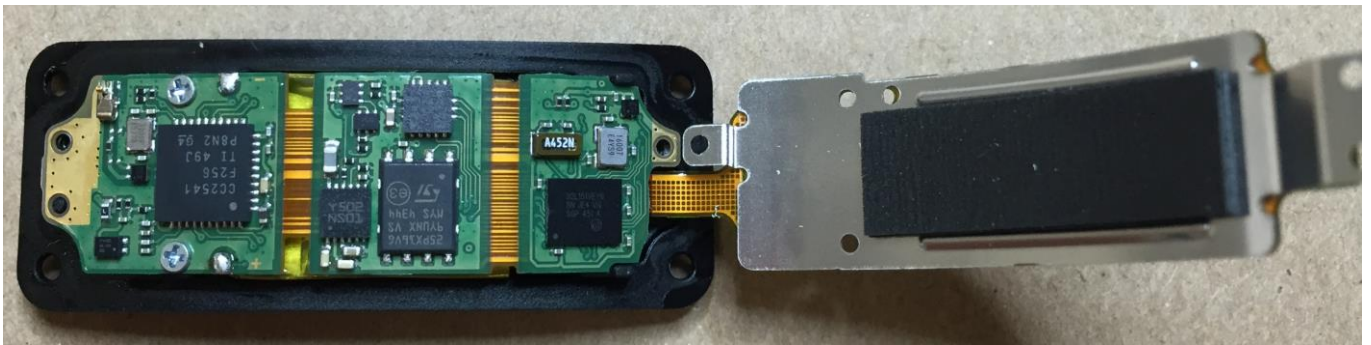
Figure 4. LED matrix module folded open.
