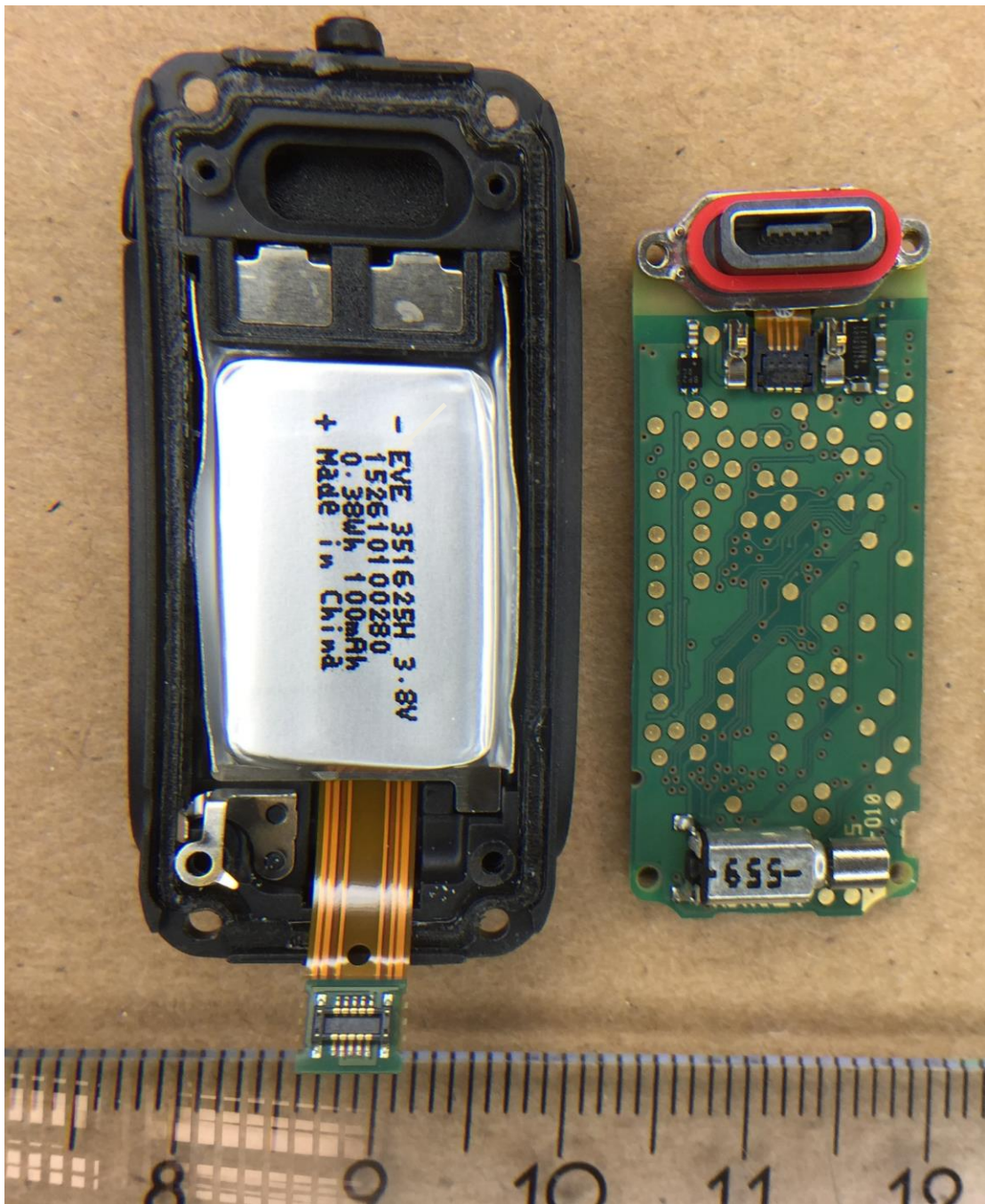
Figure 2. PWB module separated from back cover module.
