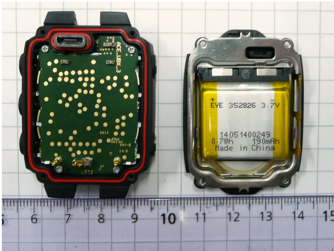
Figure 1. Back cover opened
