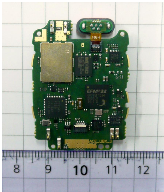
Figure 4. PWB module, top view
