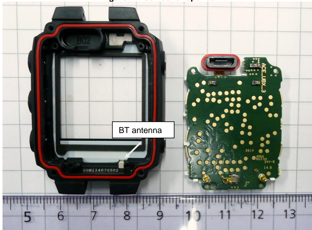
Figure 2. PWB module and front cover with LDS antennas
