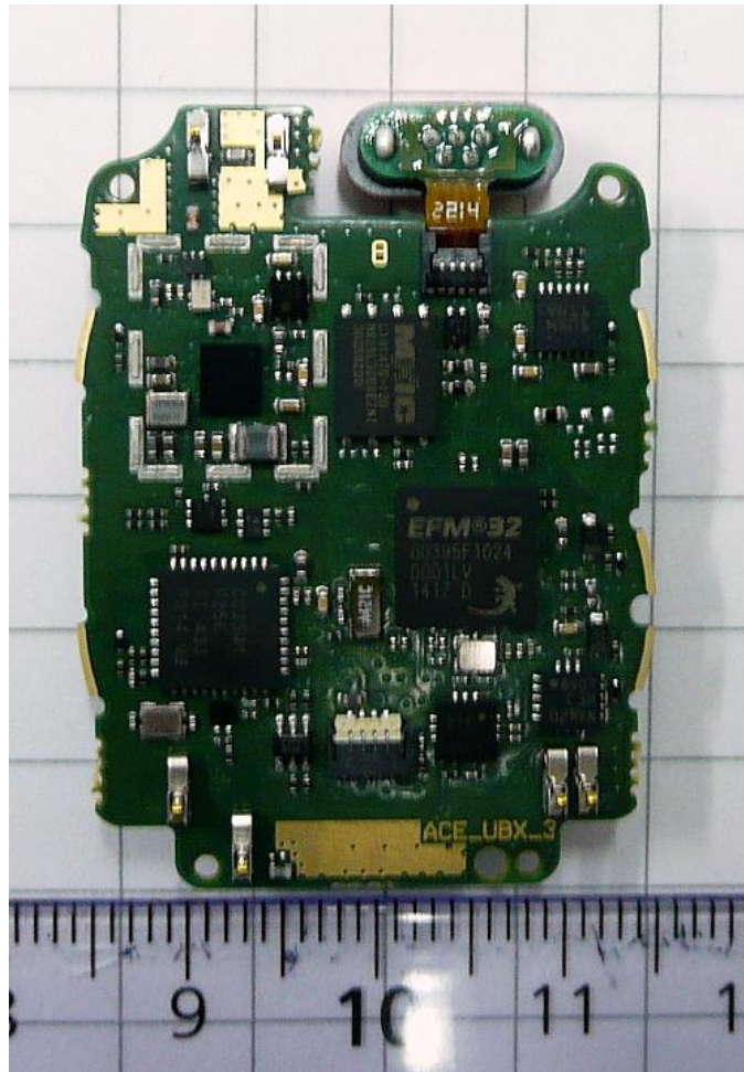
Figure 5. PWB module shield opened, top view.
