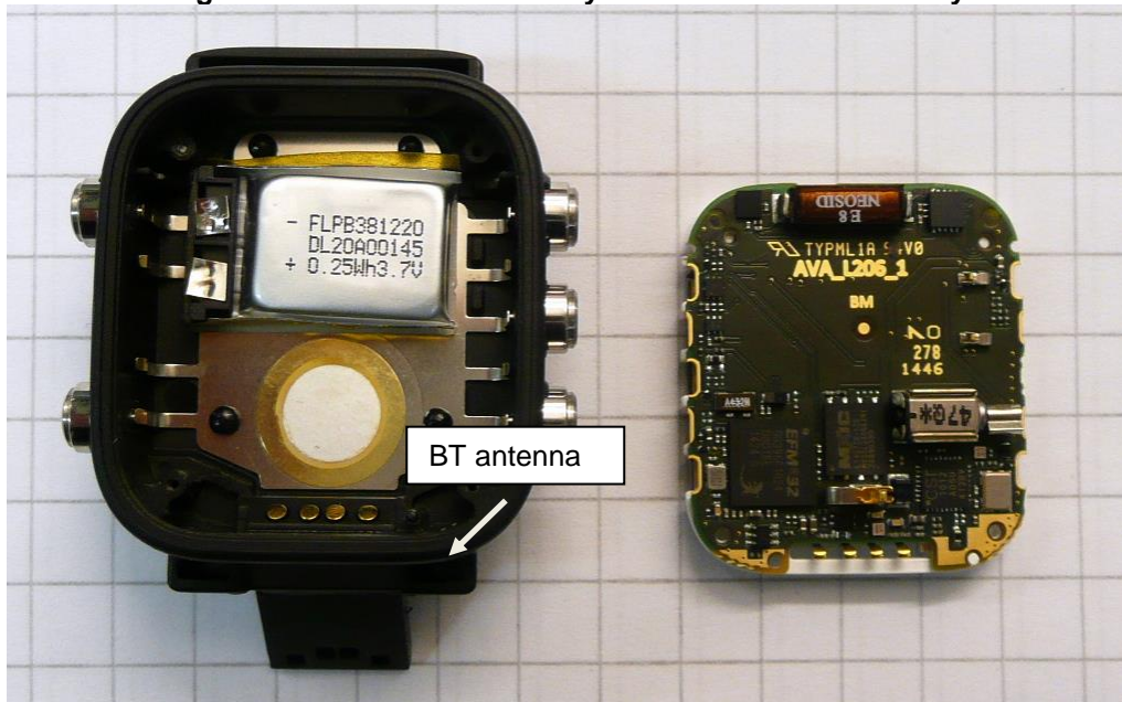
Figure 2. Back cover assembly and electronics assembly, other side
