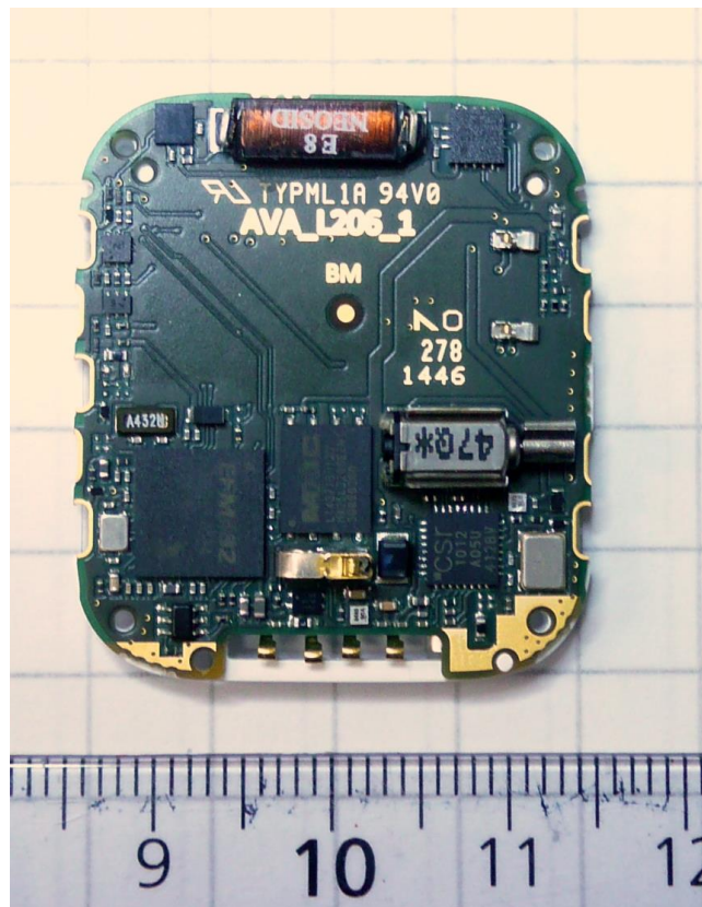
Figure 7. PWB module, bottom view
