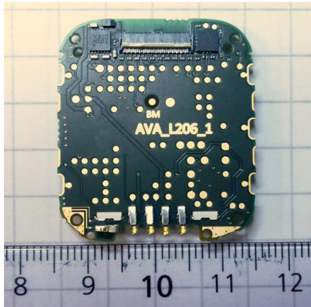
Figure 6. PWB module, top view.
