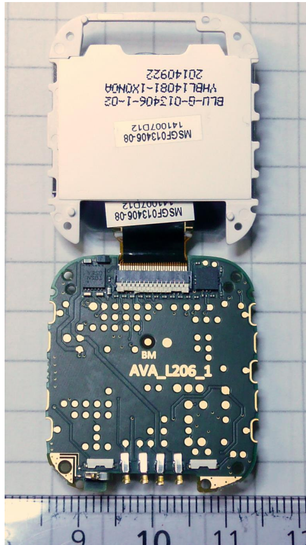
Figure 5. Display module folded open.
