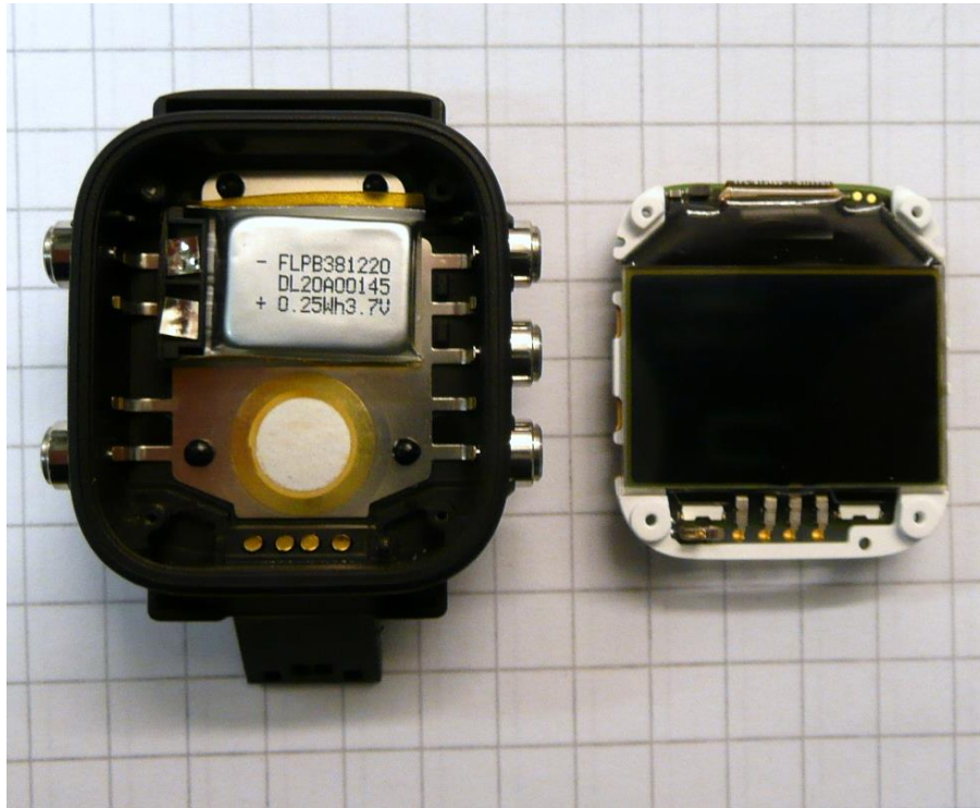
Figure 1. Back cover assembly and electronics assembly
