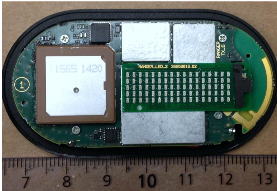
Figure 1. Electronics assembly, front case removed.
