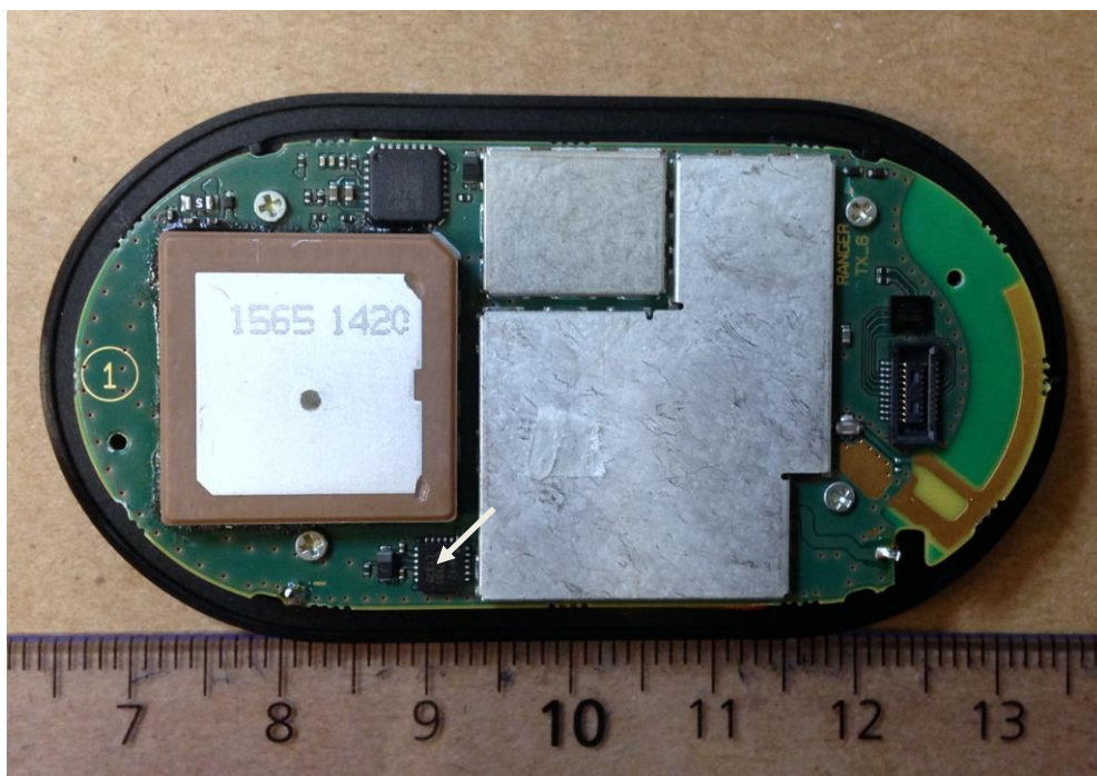
Figure 2. LED flex removed.
