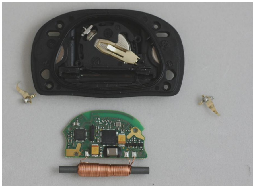
Figure 2. PWB removed from the back cover.
