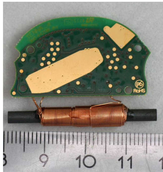
Figure 4. PWB module, bottom side.
