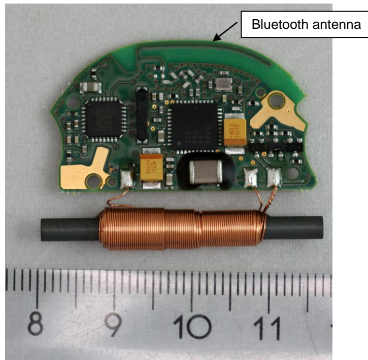
Figure 3. PWB module, top side.
