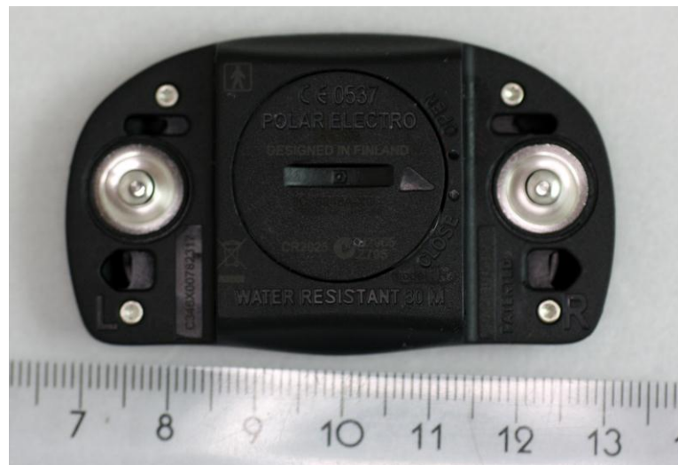
Figure 2. Back view
