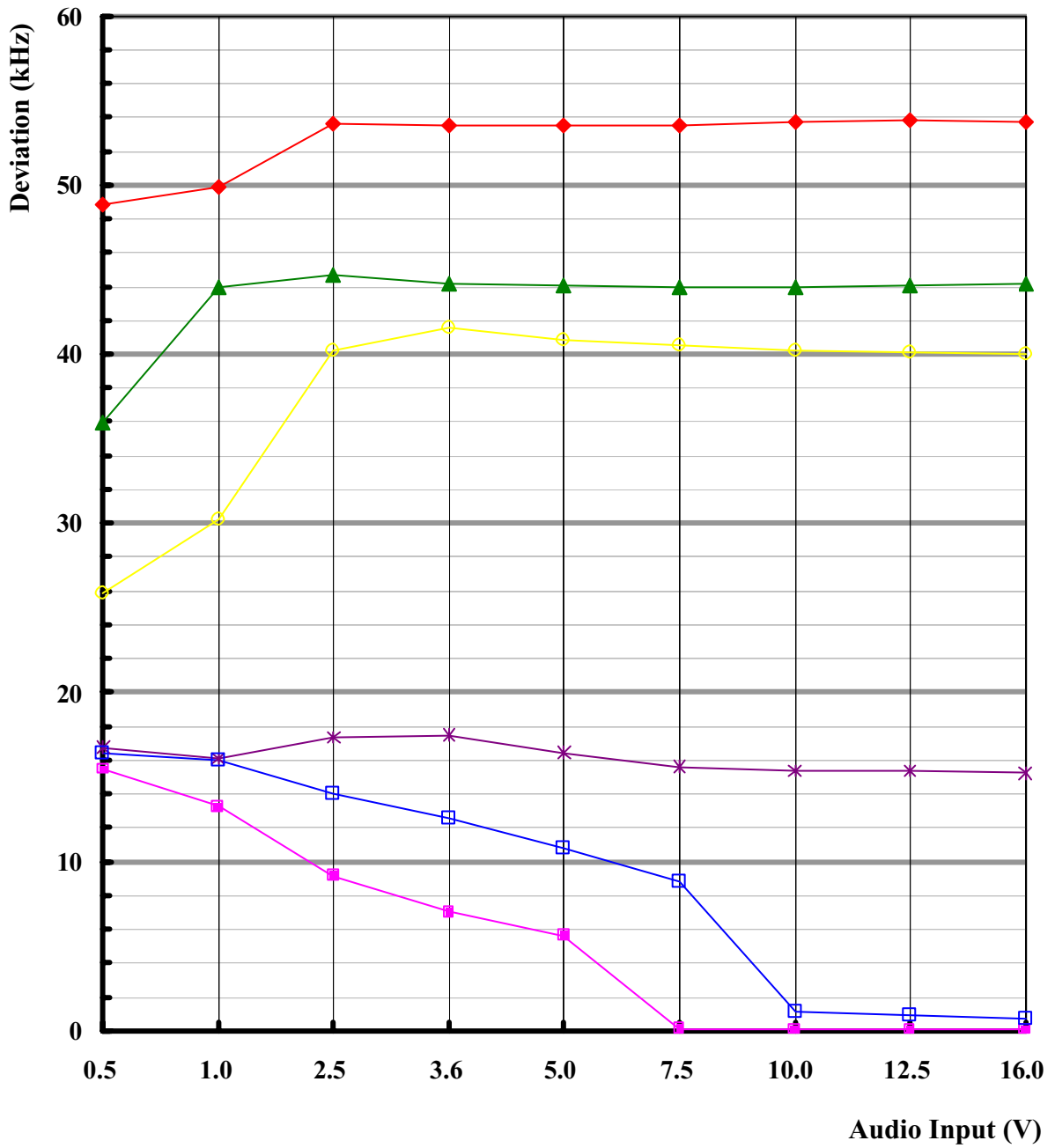
Chart 4.2 Modulation Limiting Measurement Positive
