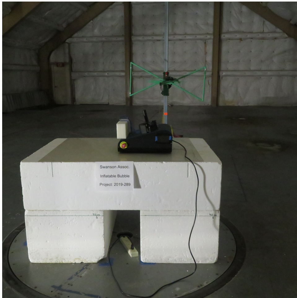
3-meter EUT set up in OATS, 30-1000MHz, front
