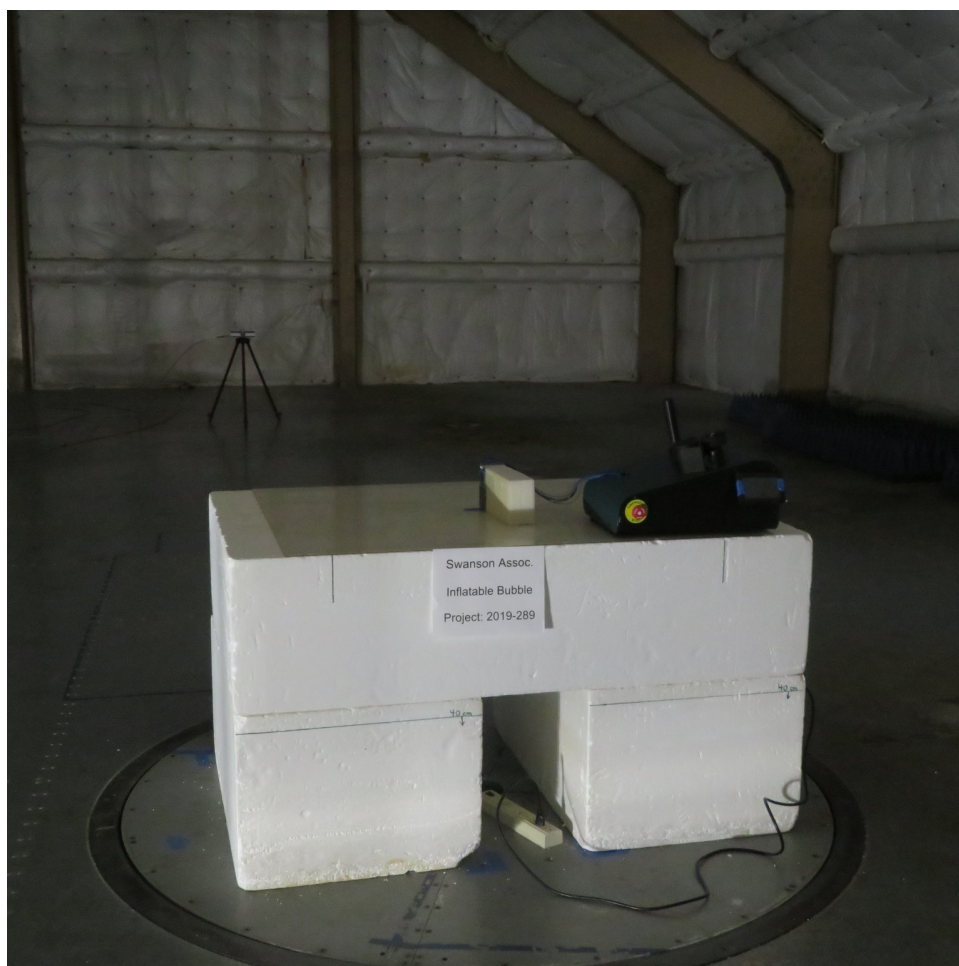
10-meter EUT set up in OATS, 9kHz – 30MHz, front
