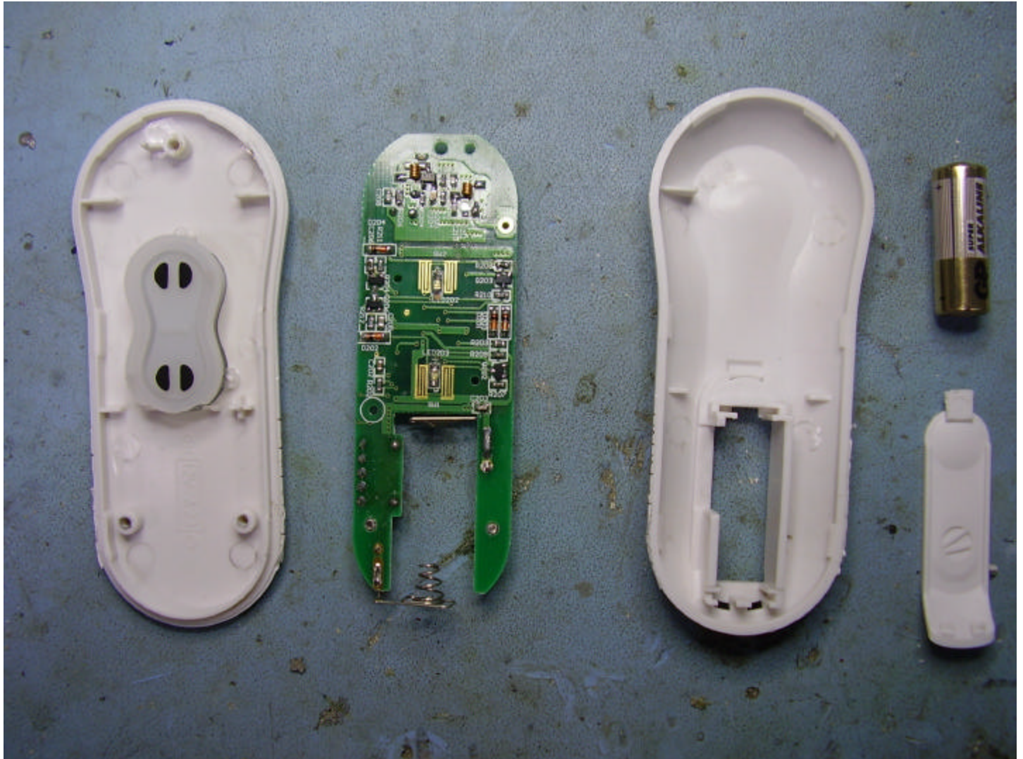
Internal Photo – Cover open showing keypad side and battery door
