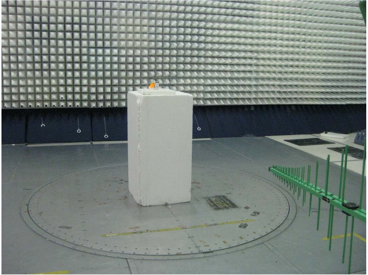
Test Setup Photo Radem 1
