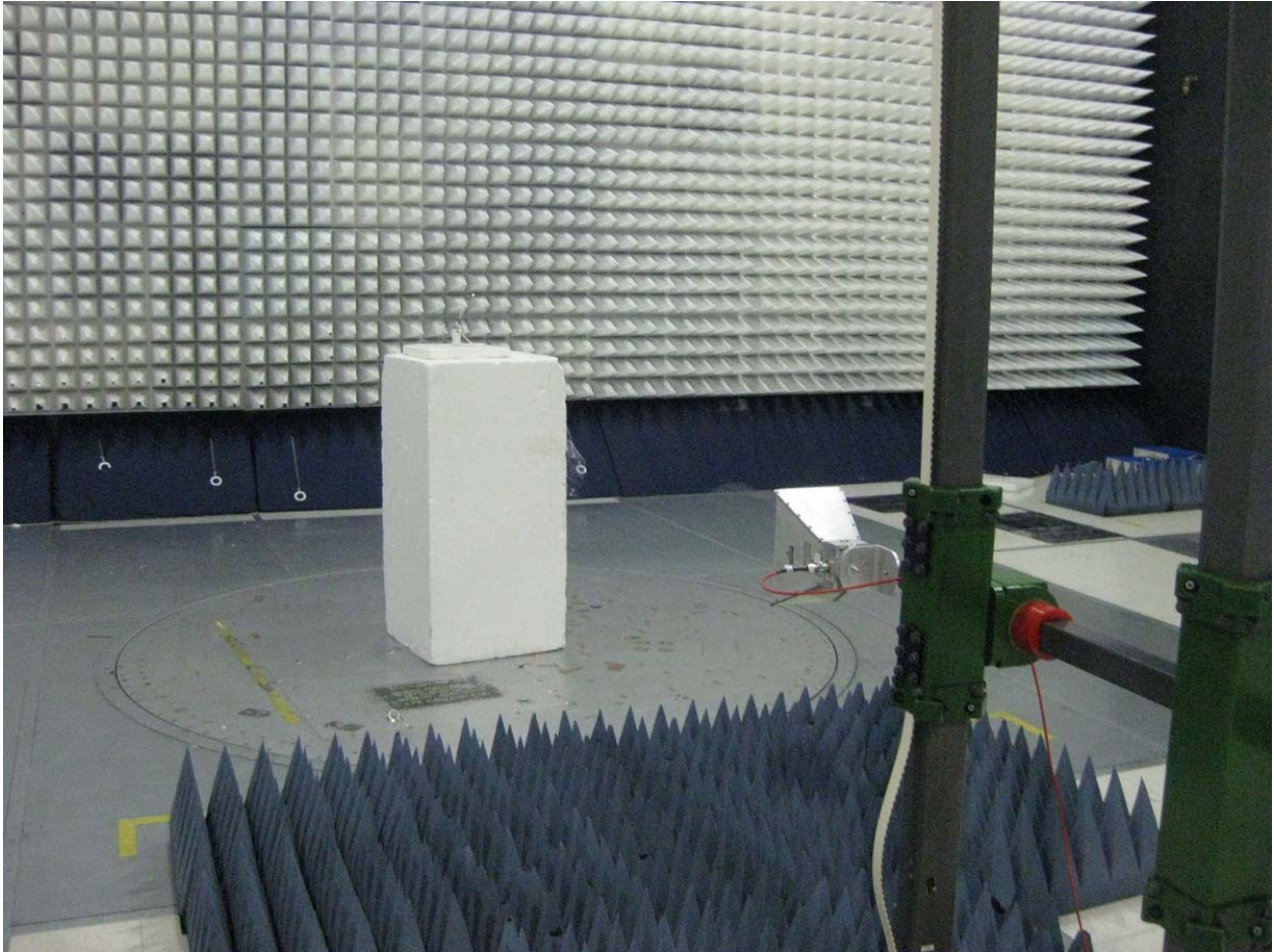
Test Setup Photo Radem Hi Freq
