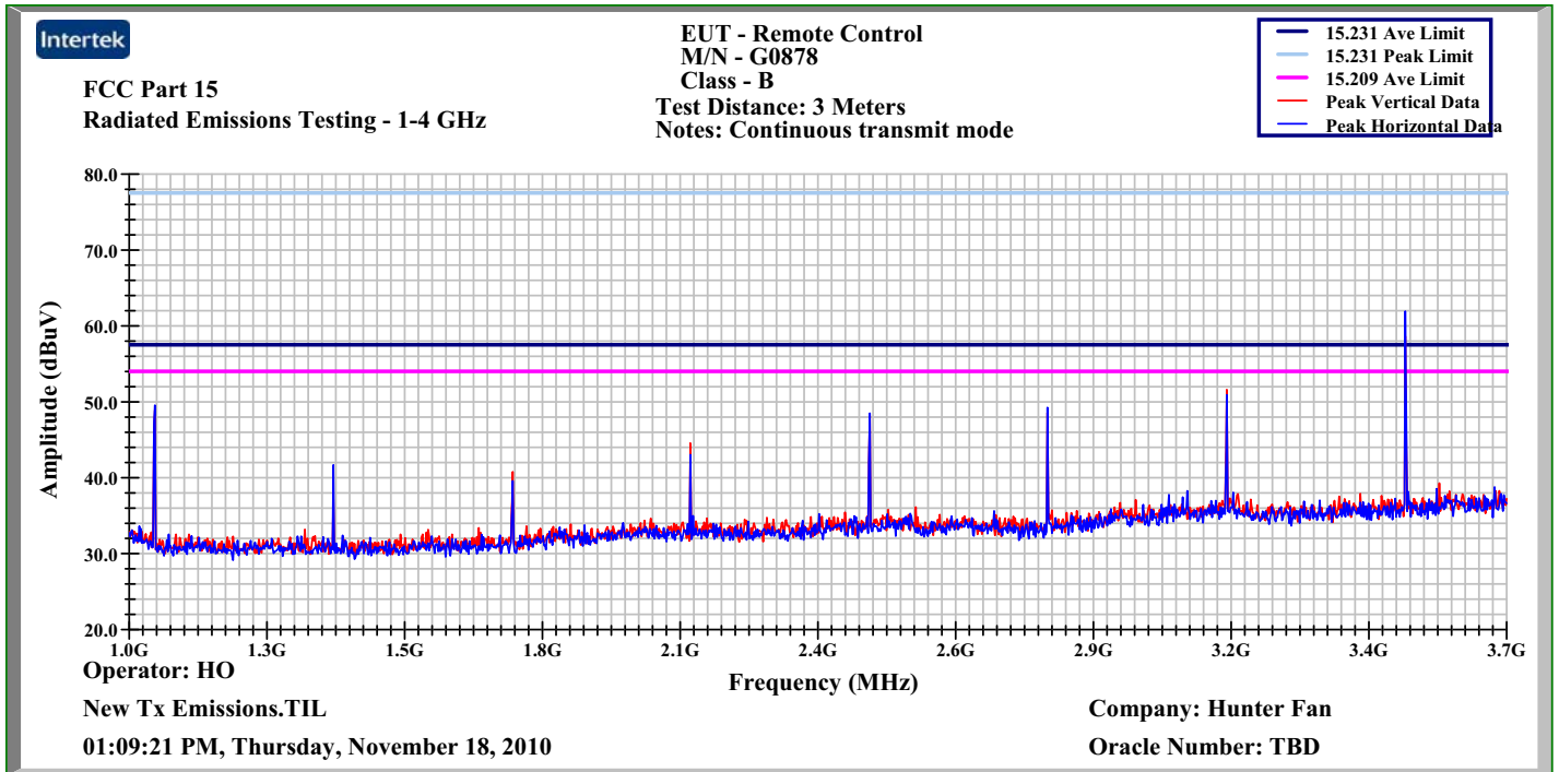
Radiated Emissions Plot - 1000-3700 MHz
