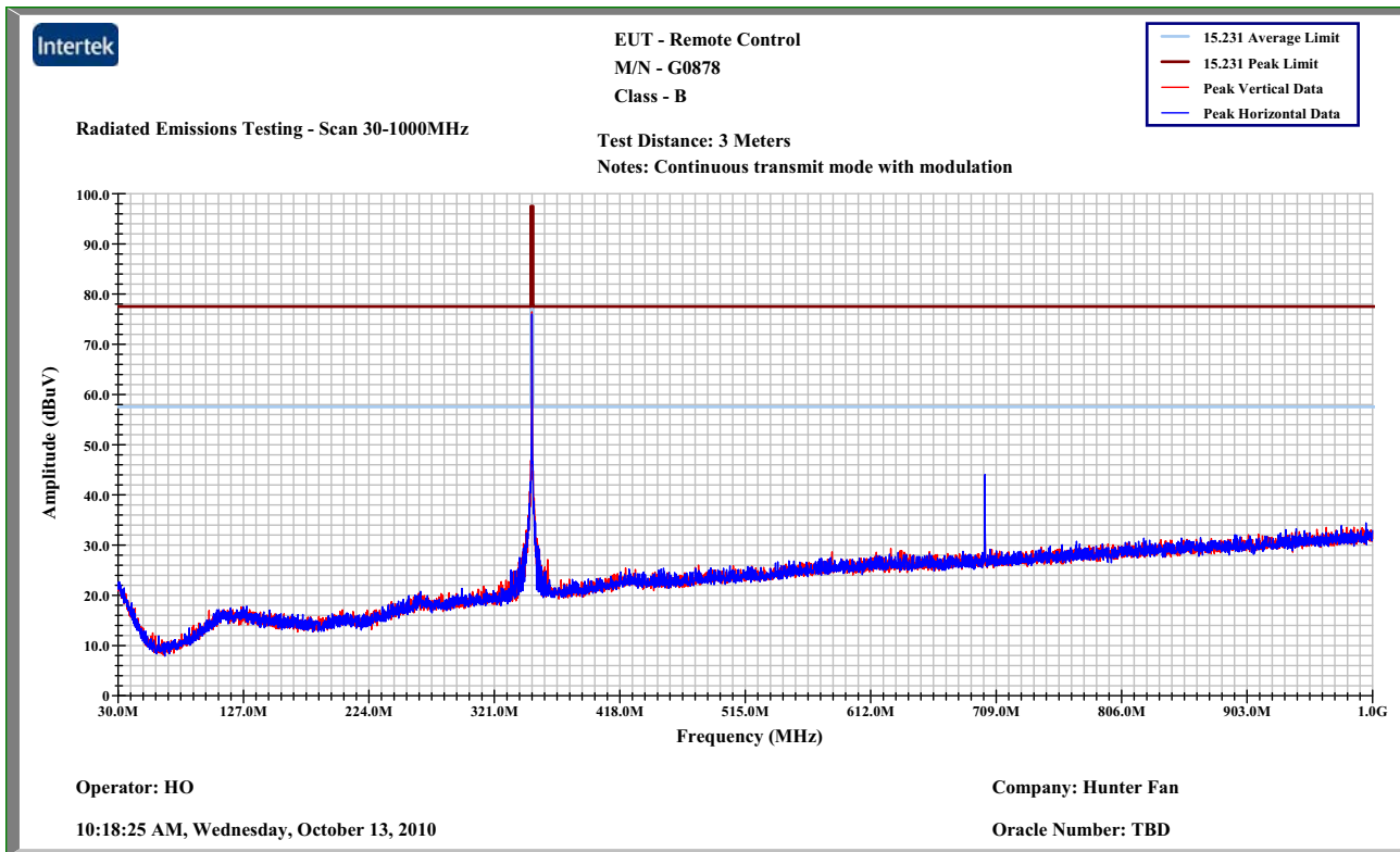
Radiated Emissions Plot - 30-1000 MHz
