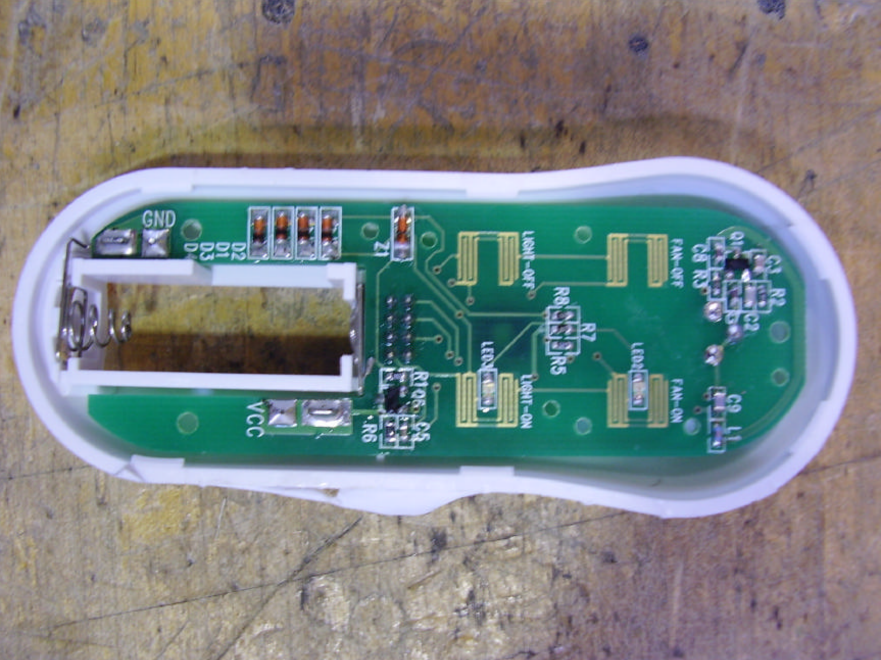
Model 27157 Transmitter – Circuit Board – Keypad Side
