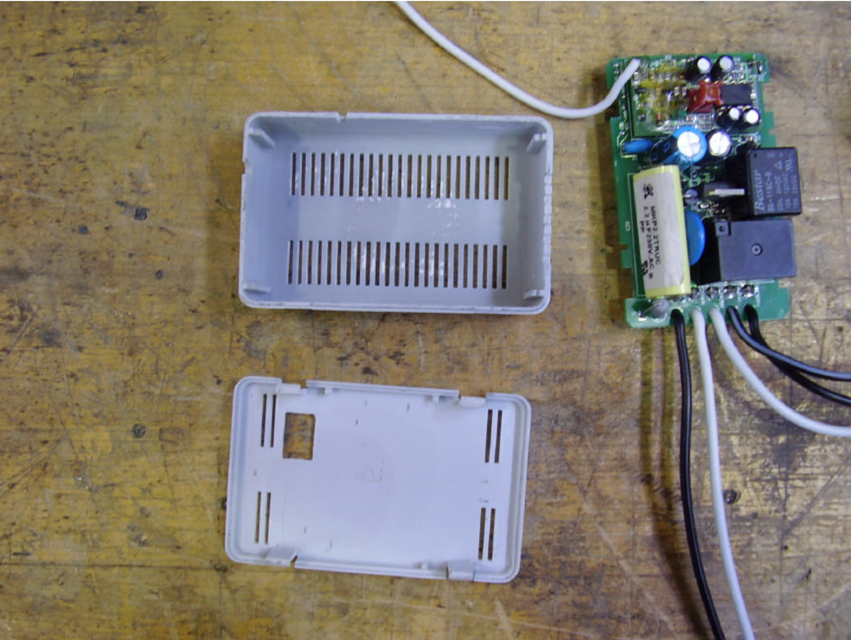
Model 27157 Receiver – Expanded – Circuit Board Assembly with Plastic Case
