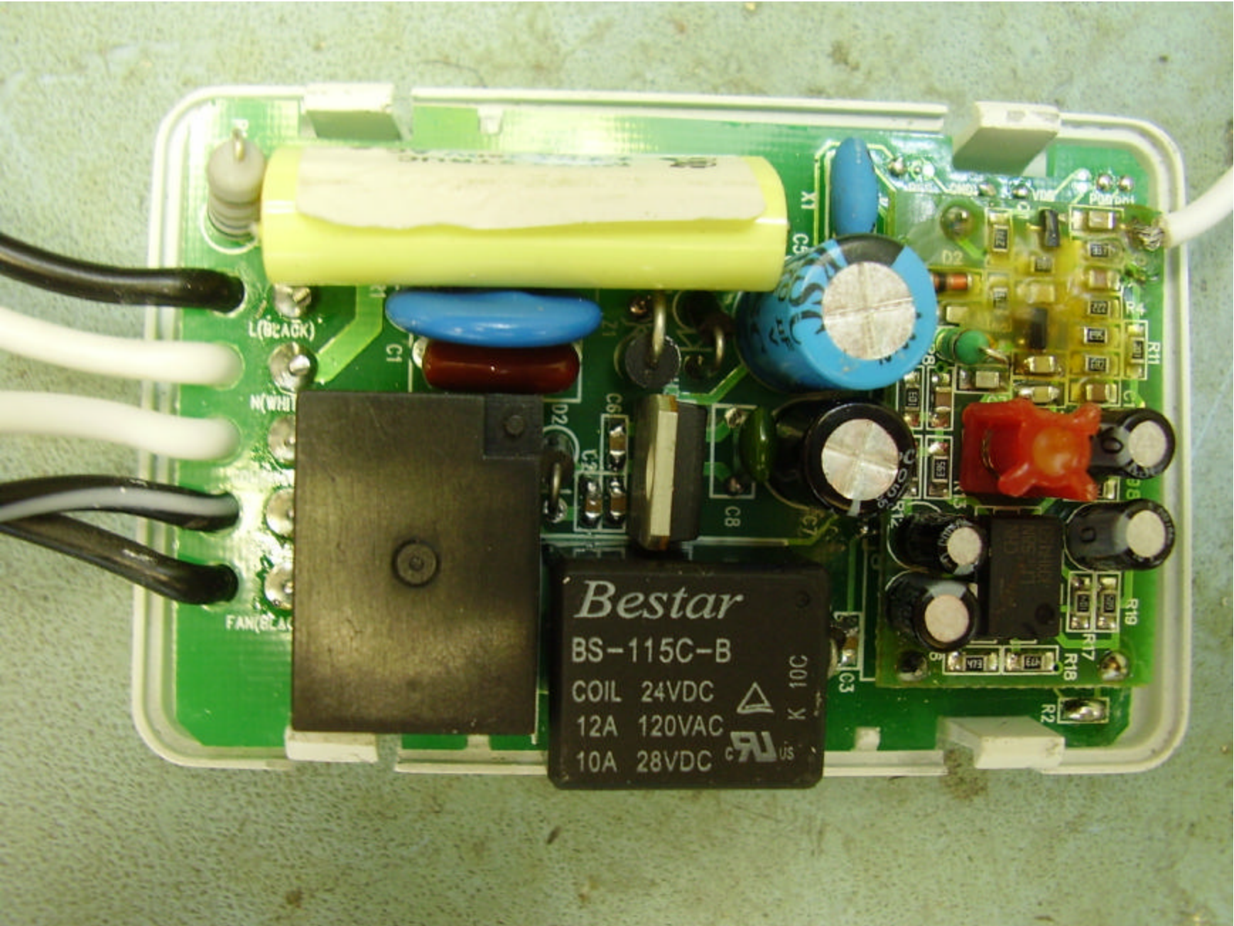
Model 27157 Receiver – Circuit Board – Component Side
