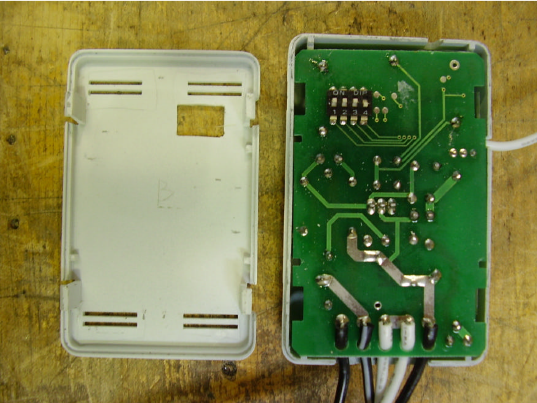
Model 27157 Receiver – Circuit Board – Solder Side
