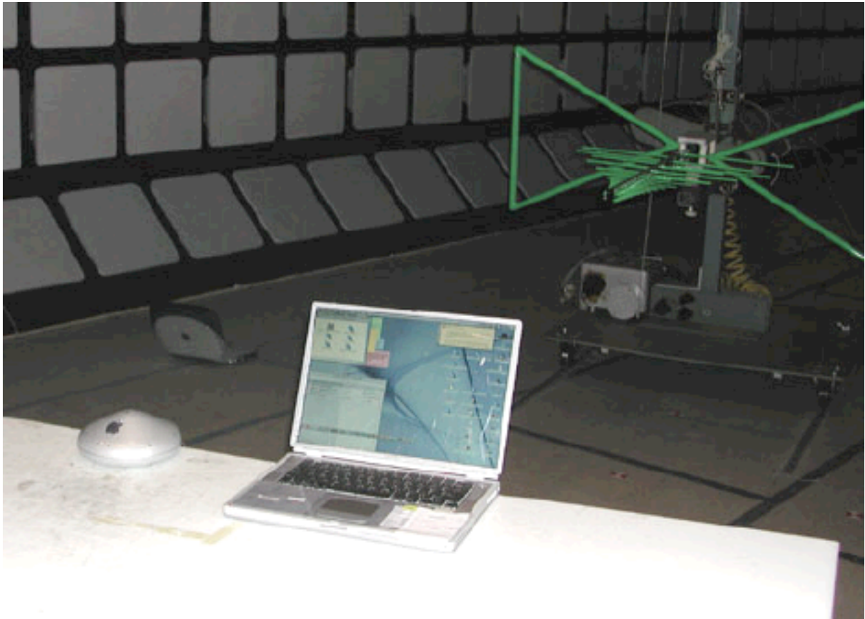
Photo 5 Radiated Emissions Test Setup below 1 GHz
