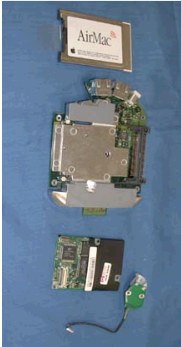
Photo 7 Apple Airport Base Station Components.
