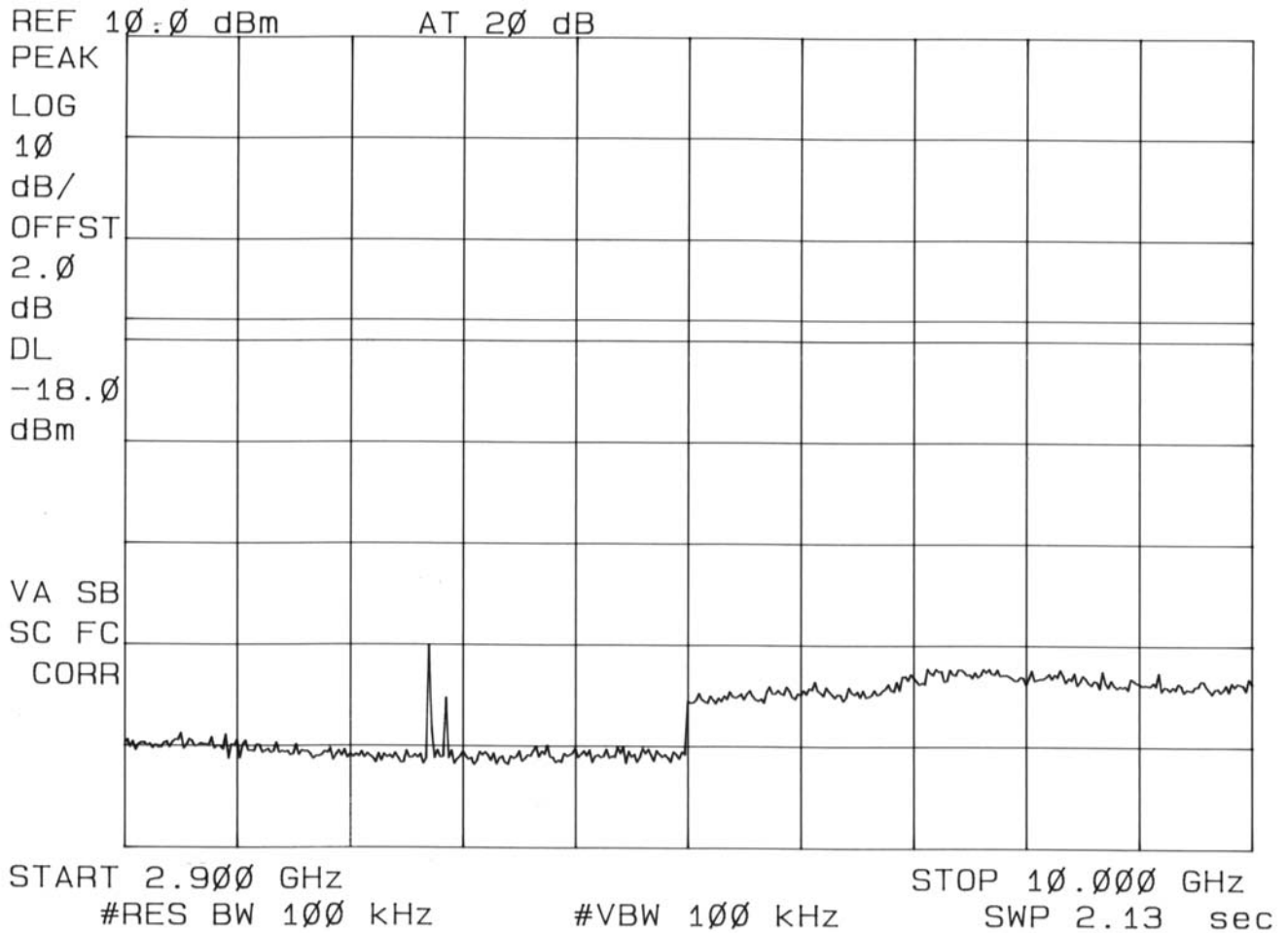
Plot 6 - Conducted emission outside restricted band.
