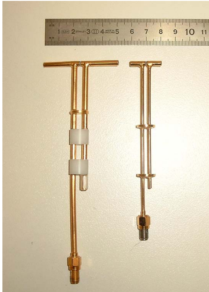
Photo 1: validation dipoles
