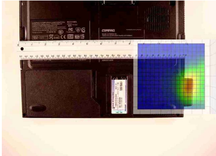
Photo 6: A 2d scan overlay giving the field strength in the first scanned plane, overlaid on a bottom side view photo of the laptop. 2d scan is that of the worst case lapheld value in channel 6, in the compaq host
