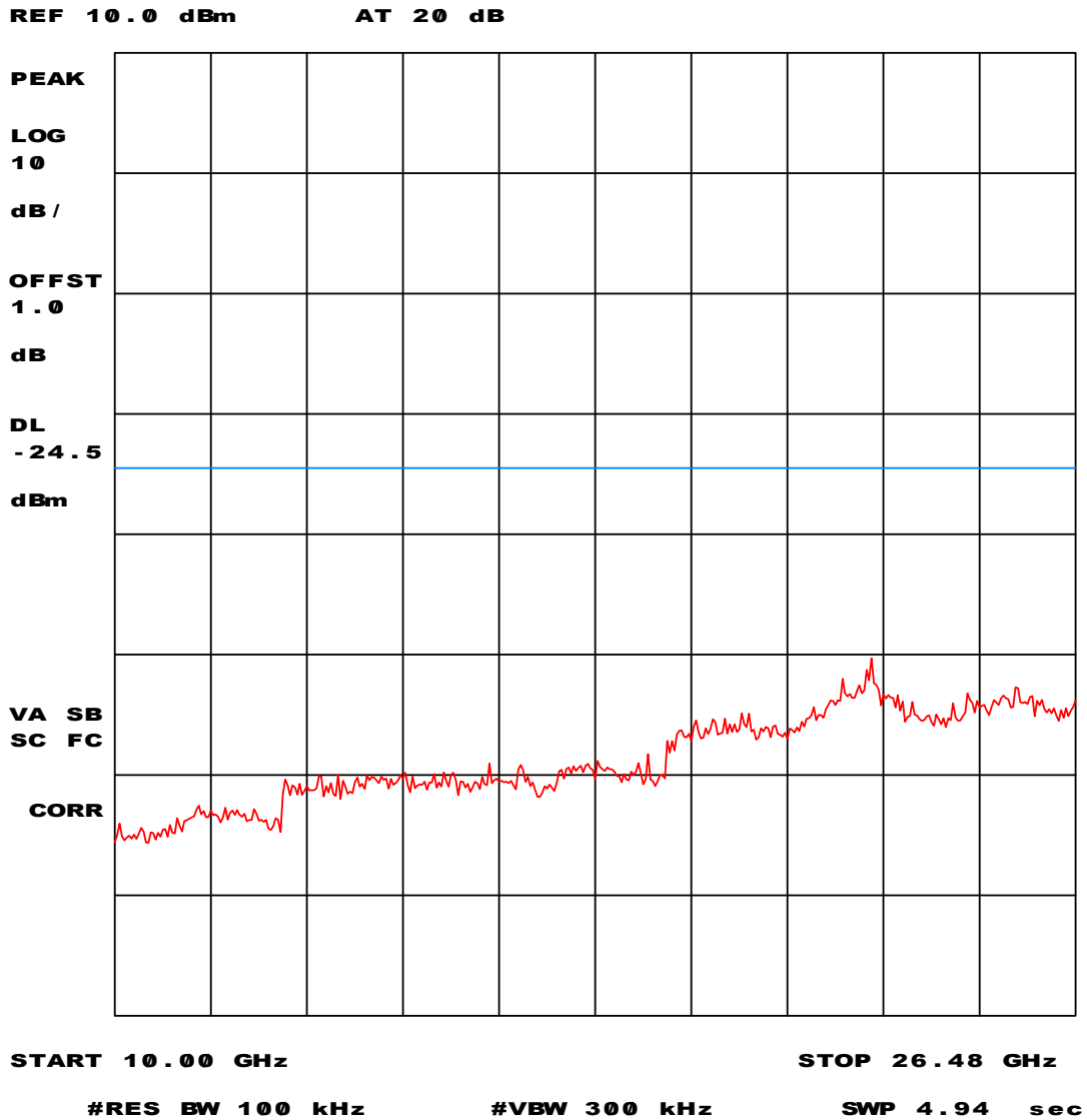
Plot 25 - Conducted emission outside restricted band (OFDM mode).
